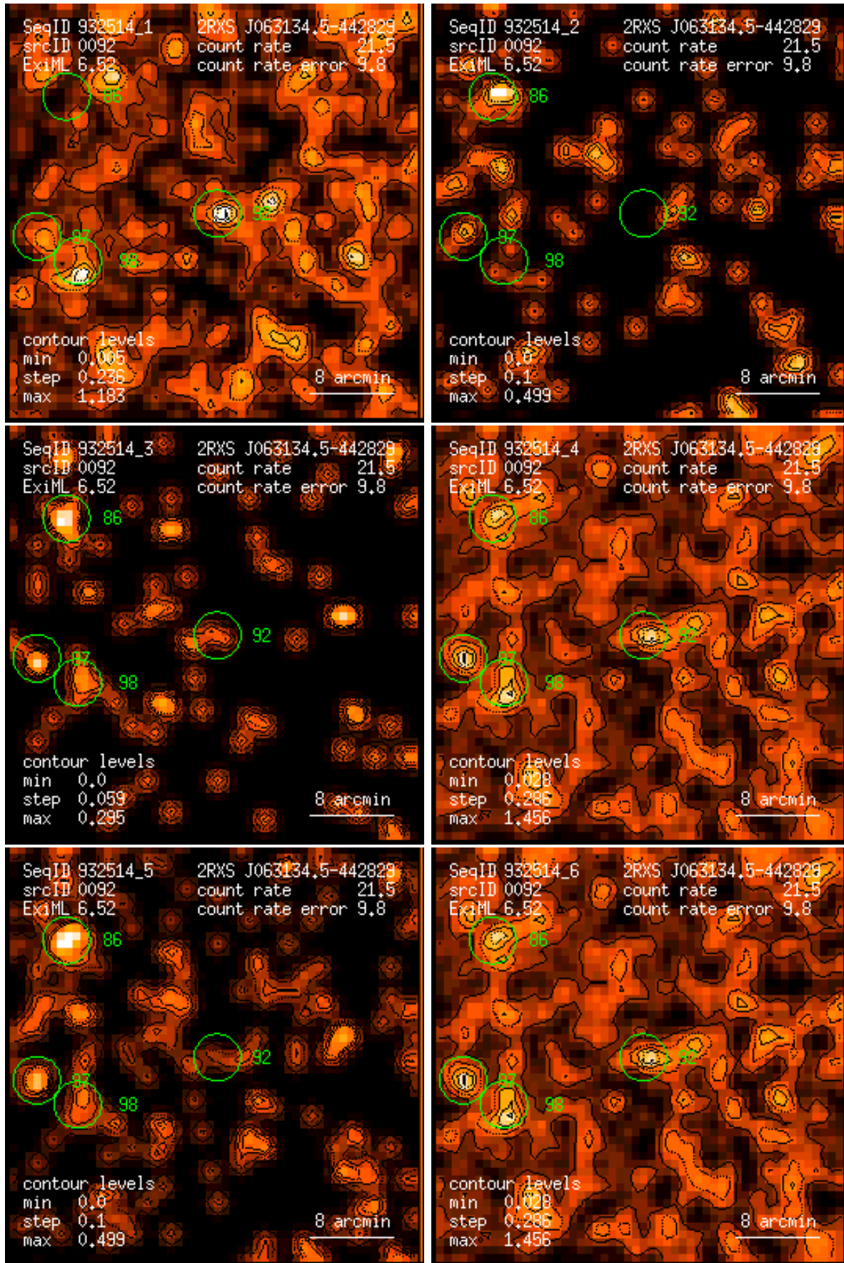
Figure 92: RASS 932514: detection 0092: band rate images, Gaussian filter: (1) PSPC channels 11 – 41, (2) 52 – 90, (3) 91 – 201, (4) 11 – 235, (5) 52 – 201, (6) 11 – 201. Broad band rates in counts/ks. Band rate contour levels in counts/ks/arcmin 2 .
