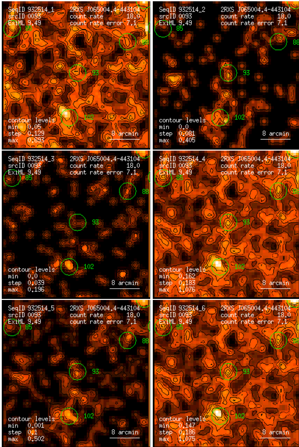
Figure 93: RASS 932514: detection 0093: band rate images, Gaussian filter: (1) PSPC channels 11 – 41, (2) 52 – 90, (3) 91 – 201, (4) 11 – 235, (5) 52 – 201, (6) 11 – 201. Broad band rates in counts/ks. Band rate contour levels in counts/ks/arcmin 2 .
