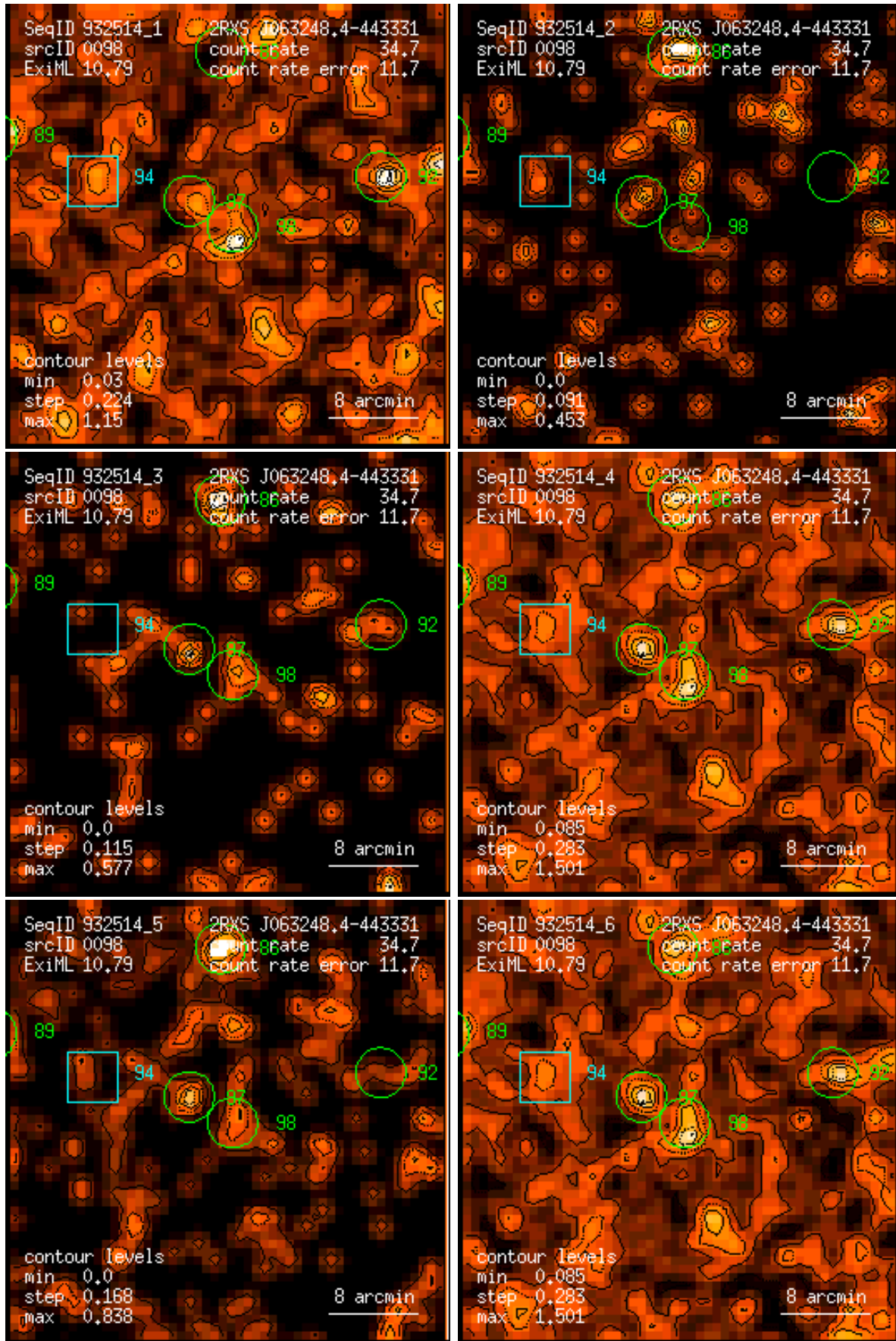
Figure 98: RASS 932514: detection 0098: band rate images, Gaussian filter: (1) PSPC channels 11 – 41, (2) 52 – 90, (3) 91 – 201, (4) 11 – 235, (5) 52 – 201, (6) 11 – 201. Broad band rates in counts/ks. Band rate contour levels in counts/ks/arcmin 2 .
