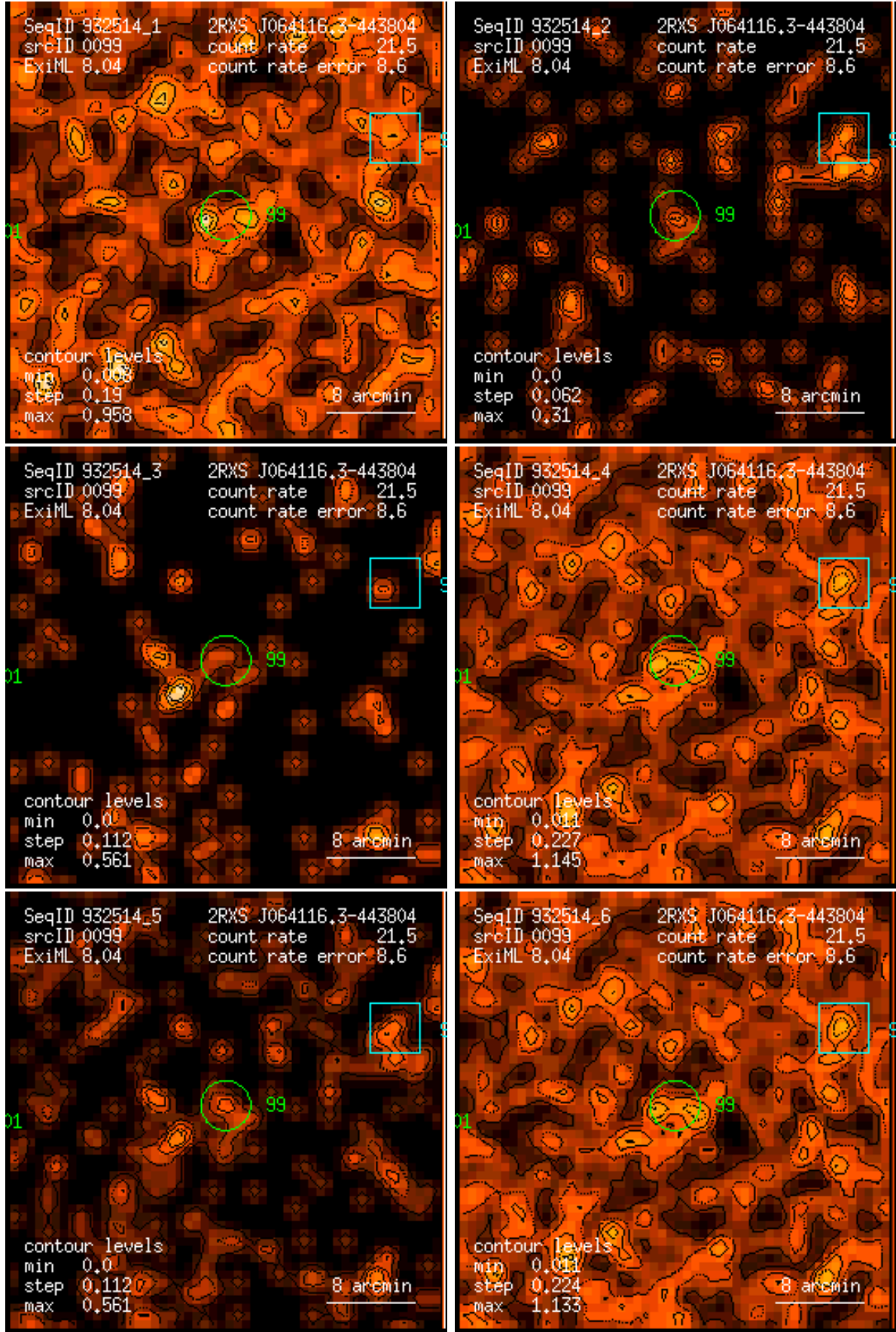
Figure 99: RASS 932514: detection 0099: band rate images, Gaussian filter: (1) PSPC channels 11 – 41, (2) 52 – 90, (3) 91 – 201, (4) 11 – 235, (5) 52 – 201, (6) 11 – 201. Broad band rates in counts/ks. Band rate contour levels in counts/ks/arcmin 2 .
