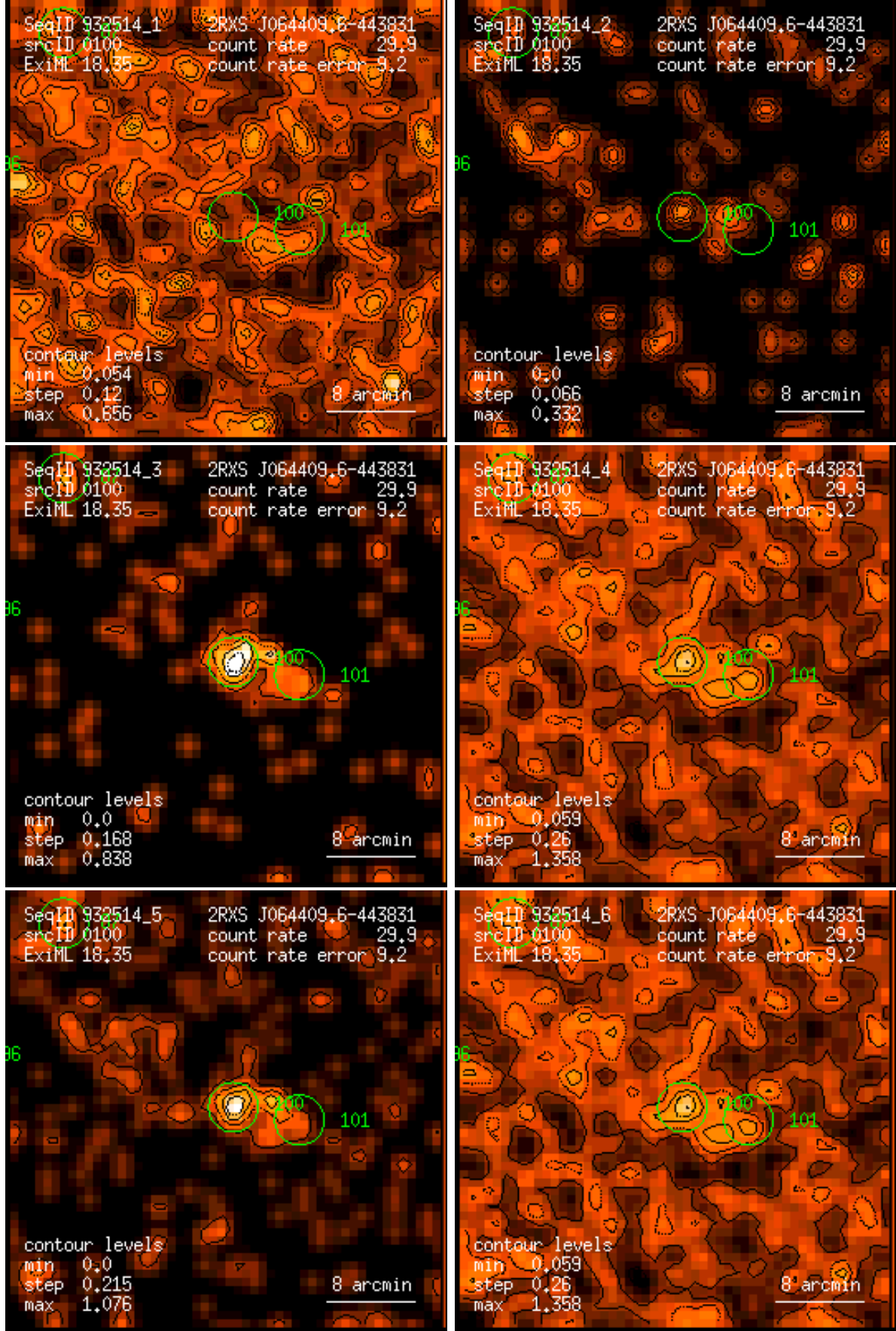
Figure 100: RASS 932514: detection 0100: band rate images, Gaussian filter: (1) PSPC channels 11 – 41, (2) 52 – 90, (3) 91 – 201, (4) 11 – 235, (5) 52 – 201, (6) 11 – 201. Broad band rates in counts/ks. Band rate contour levels in counts/ks/arcmin 2 .
