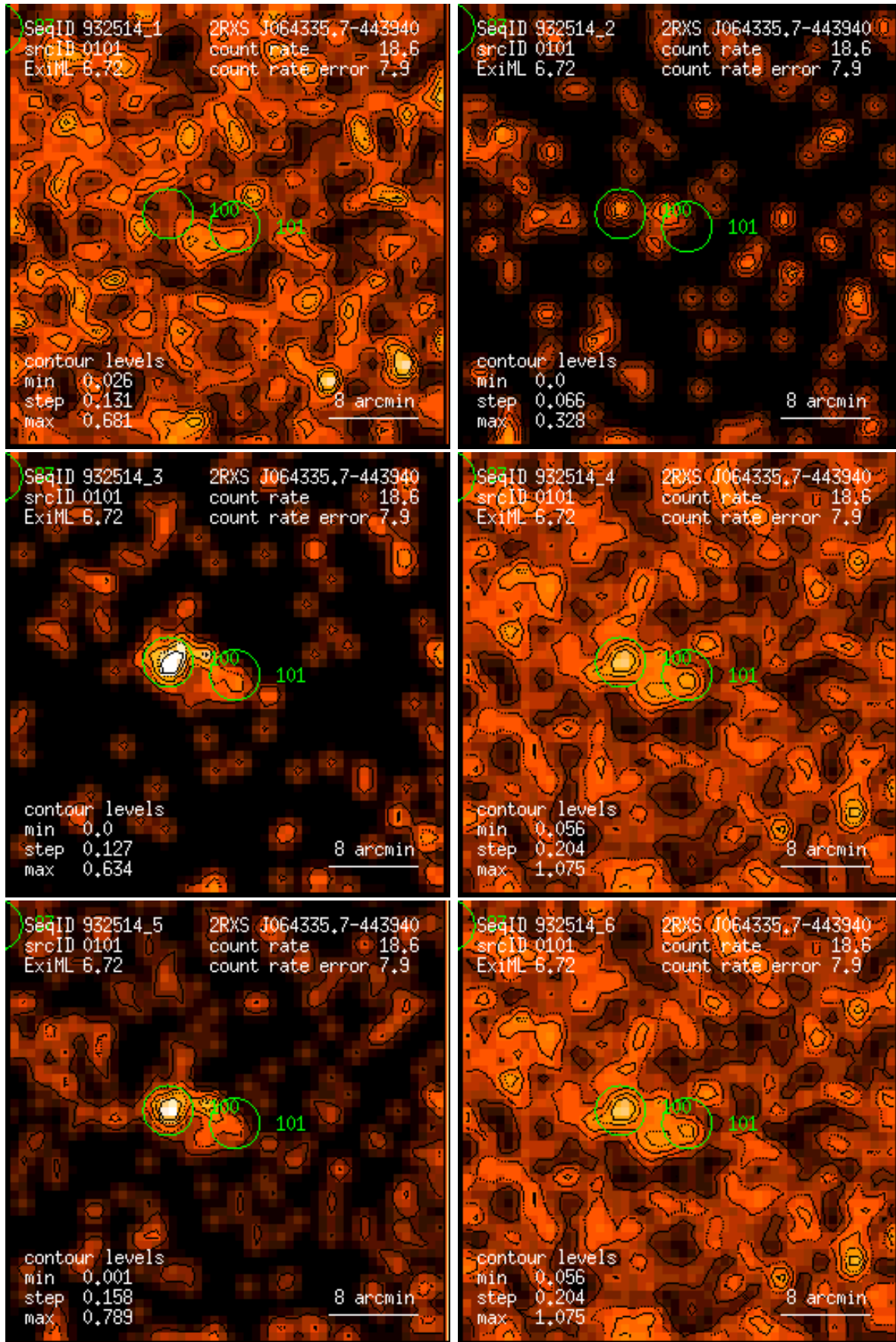
Figure 101: RASS 932514: detection 0101: band rate images, Gaussian filter: (1) PSPC channels 11 – 41, (2) 52 – 90, (3) 91 – 201, (4) 11 – 235, (5) 52 – 201, (6) 11 – 201. Broad band rates in counts/ks. Band rate contour levels in counts/ks/arcmin 2 .
