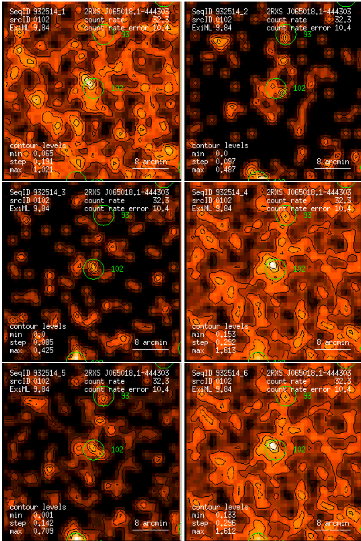
Figure 102: RASS 932514: detection 0102: band rate images, Gaussian filter: (1) PSPC channels 11 – 41, (2) 52 – 90, (3) 91 – 201, (4) 11 – 235, (5) 52 – 201, (6) 11 – 201. Broad band rates in counts/ks. Band rate contour levels in counts/ks/arcmin 2 .
