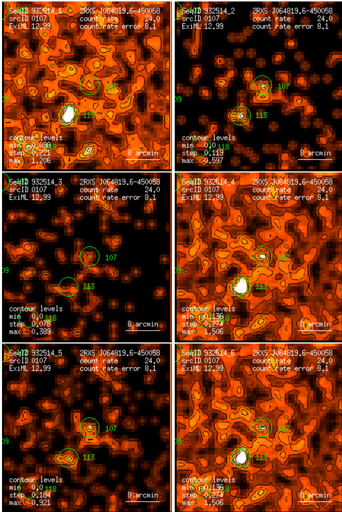
Figure 107: RASS 932514: detection 0107: band rate images, Gaussian filter: (1) PSPC channels 11 – 41, (2) 52 – 90, (3) 91 – 201, (4) 11 – 235, (5) 52 – 201, (6) 11 – 201. Broad band rates in counts/ks. Band rate contour levels in counts/ks/arcmin 2 .
