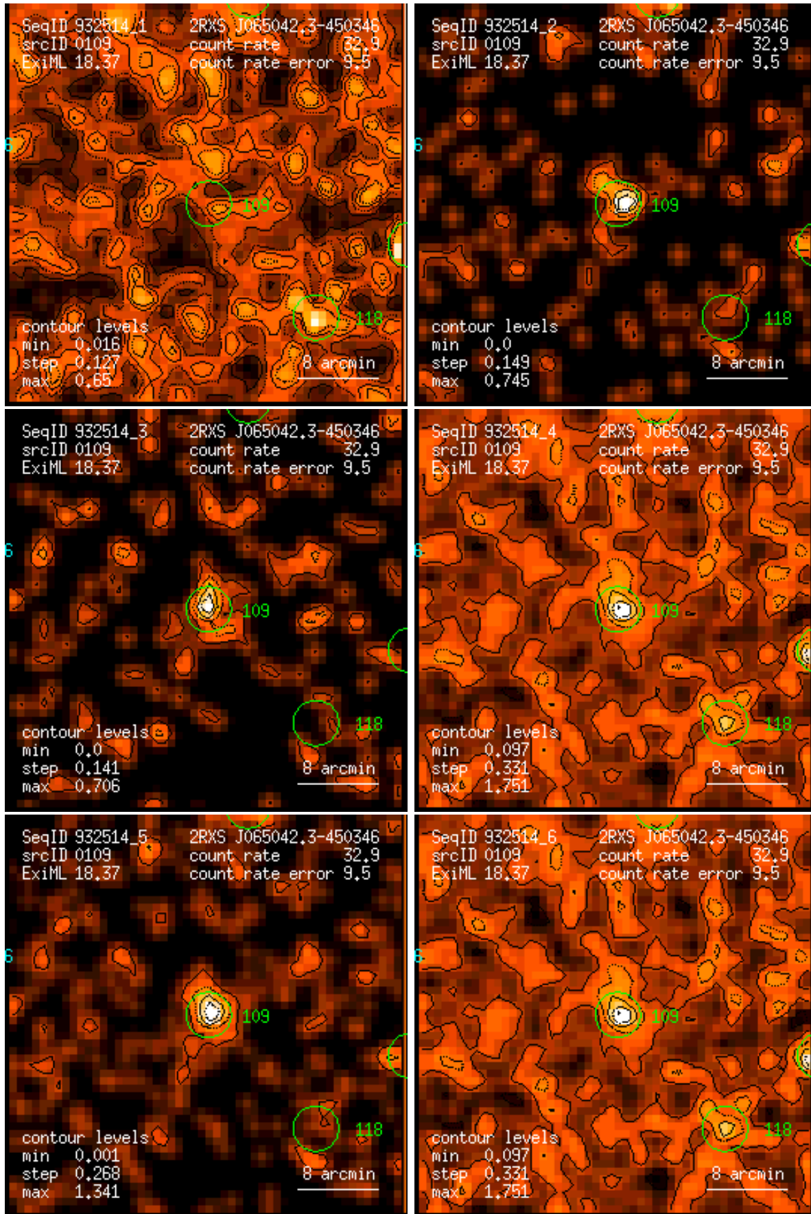
Figure 109: RASS 932514: detection 0109: band rate images, Gaussian filter: (1) PSPC channels 11 – 41, (2) 52 – 90, (3) 91 – 201, (4) 11 – 235, (5) 52 – 201, (6) 11 – 201. Broad band rates in counts/ks. Band rate contour levels in counts/ks/arcmin 2 .
