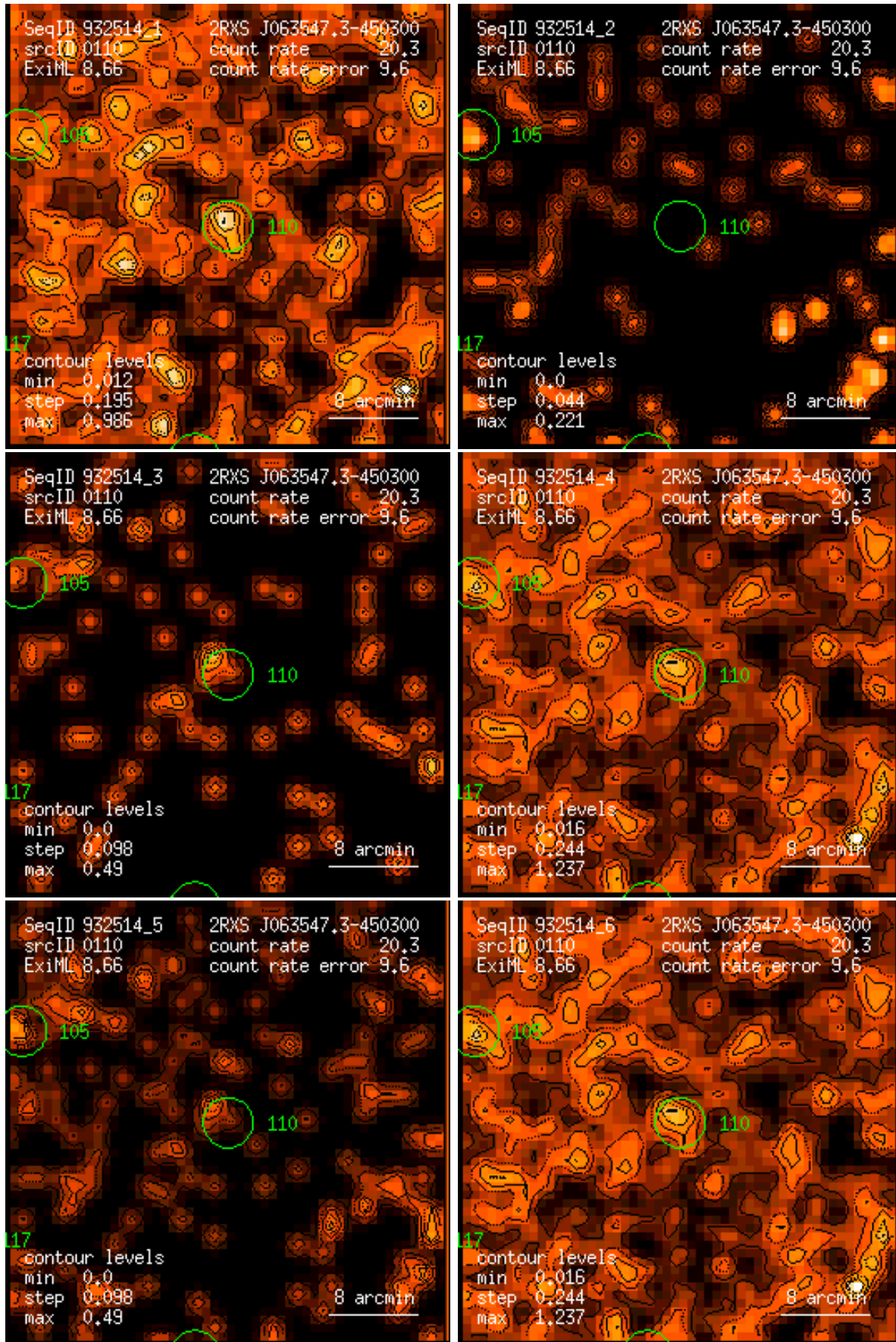
Figure 110: RASS 932514: detection 0110: band rate images, Gaussian filter: (1) PSPC channels 11 – 41, (2) 52 – 90, (3) 91 – 201, (4) 11 – 235, (5) 52 – 201, (6) 11 – 201. Broad band rates in counts/ks. Band rate contour levels in counts/ks/arcmin 2 .
