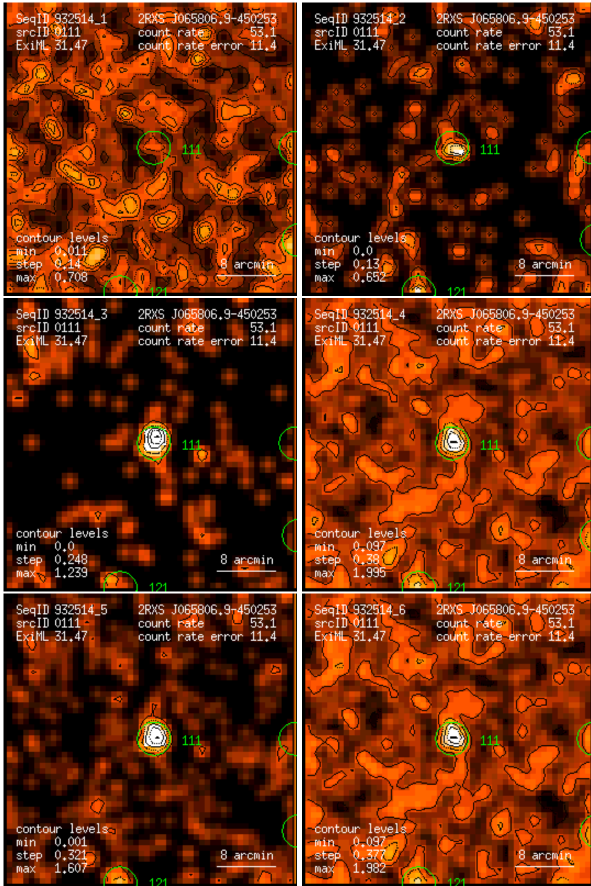
Figure 111: RASS 932514: detection 0111: band rate images, Gaussian filter: (1) PSPC channels 11 – 41, (2) 52 – 90, (3) 91 – 201, (4) 11 – 235, (5) 52 – 201, (6) 11 – 201. Broad band rates in counts/ks. Band rate contour levels in counts/ks/arcmin 2 .
