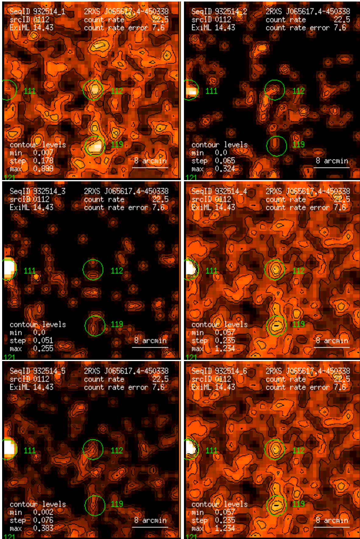
Figure 112: RASS 932514: detection 0112: band rate images, Gaussian filter: (1) PSPC channels 11 – 41, (2) 52 – 90, (3) 91 – 201, (4) 11 – 235, (5) 52 – 201, (6) 11 – 201. Broad band rates in counts/ks. Band rate contour levels in counts/ks/arcmin 2 .
