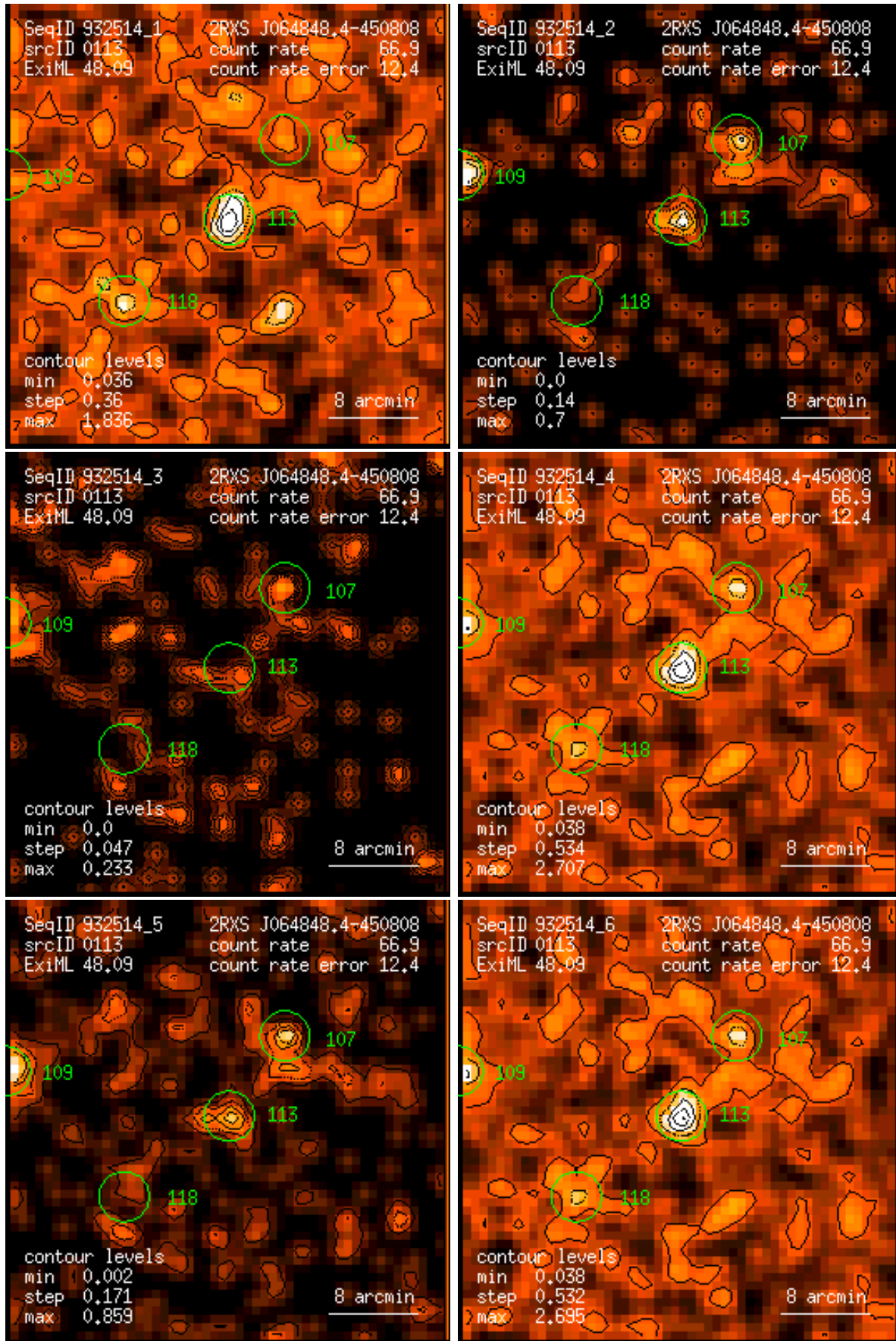
Figure 113: RASS 932514: detection 0113: band rate images, Gaussian filter: (1) PSPC channels 11 – 41, (2) 52 – 90, (3) 91 – 201, (4) 11 – 235, (5) 52 – 201, (6) 11 – 201. Broad band rates in counts/ks. Band rate contour levels in counts/ks/arcmin 2 .
