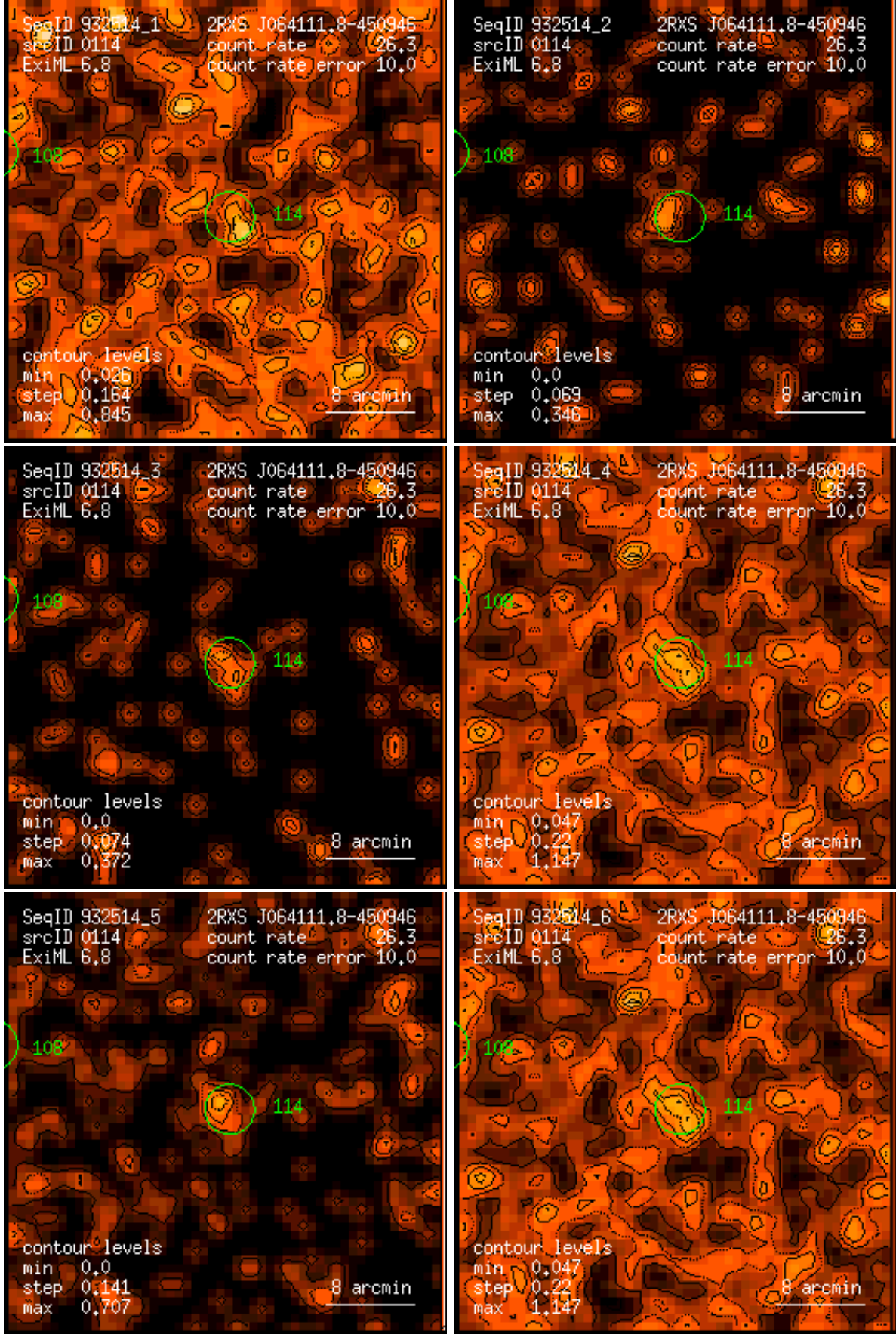
Figure 114: RASS 932514: detection 0114: band rate images, Gaussian filter: (1) PSPC channels 11 – 41, (2) 52 – 90, (3) 91 – 201, (4) 11 – 235, (5) 52 – 201, (6) 11 – 201. Broad band rates in counts/ks. Band rate contour levels in counts/ks/arcmin 2 .
