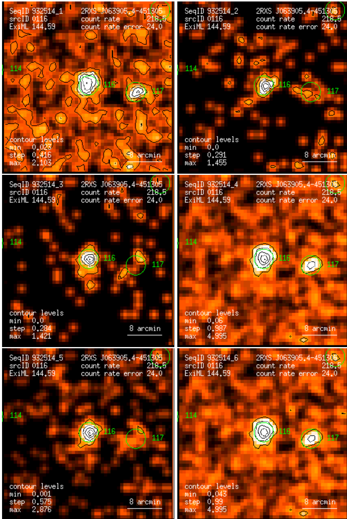
Figure 116: RASS 932514: detection 0116: band rate images, Gaussian filter: (1) PSPC channels 11 – 41, (2) 52 – 90, (3) 91 – 201, (4) 11 – 235, (5) 52 – 201, (6) 11 – 201. Broad band rates in counts/ks. Band rate contour levels in counts/ks/arcmin 2 .
