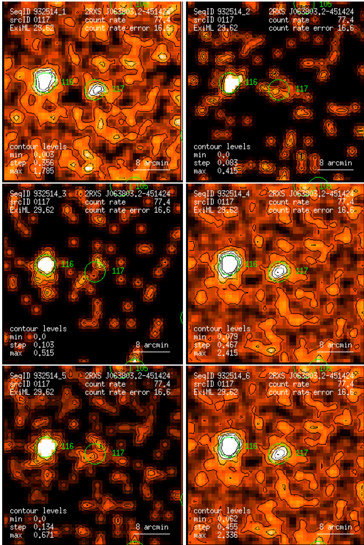
Figure 117: RASS 932514: detection 0117: band rate images, Gaussian filter: (1) PSPC channels 11 – 41, (2) 52 – 90, (3) 91 – 201, (4) 11 – 235, (5) 52 – 201, (6) 11 – 201. Broad band rates in counts/ks. Band rate contour levels in counts/ks/arcmin 2 .
