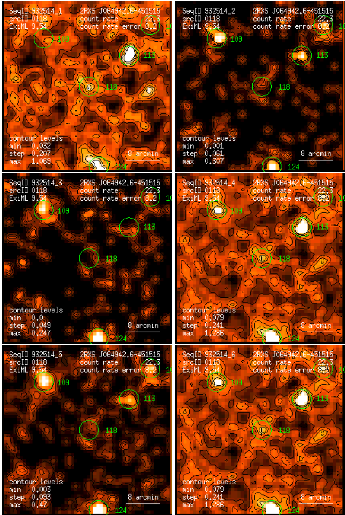
Figure 118: RASS 932514: detection 0118: band rate images, Gaussian filter: (1) PSPC channels 11 – 41, (2) 52 – 90, (3) 91 – 201, (4) 11 – 235, (5) 52 – 201, (6) 11 – 201. Broad band rates in counts/ks. Band rate contour levels in counts/ks/arcmin 2 .
