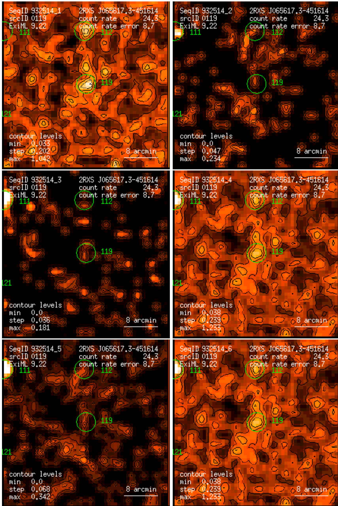
Figure 119: RASS 932514: detection 0119: band rate images, Gaussian filter: (1) PSPC channels 11 – 41, (2) 52 – 90, (3) 91 – 201, (4) 11 – 235, (5) 52 – 201, (6) 11 – 201. Broad band rates in counts/ks. Band rate contour levels in counts/ks/arcmin 2 .
