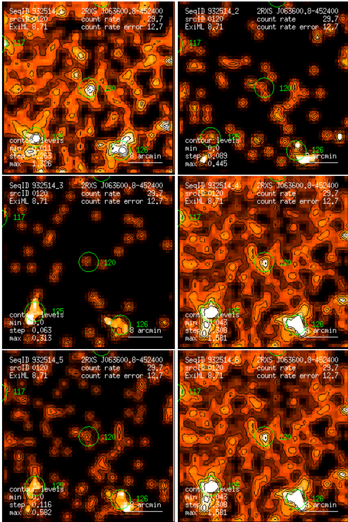
Figure 120: RASS 932514: detection 0120: band rate images, Gaussian filter: (1) PSPC channels 11 – 41, (2) 52 – 90, (3) 91 – 201, (4) 11 – 235, (5) 52 – 201, (6) 11 – 201. Broad band rates in counts/ks. Band rate contour levels in counts/ks/arcmin 2 .
