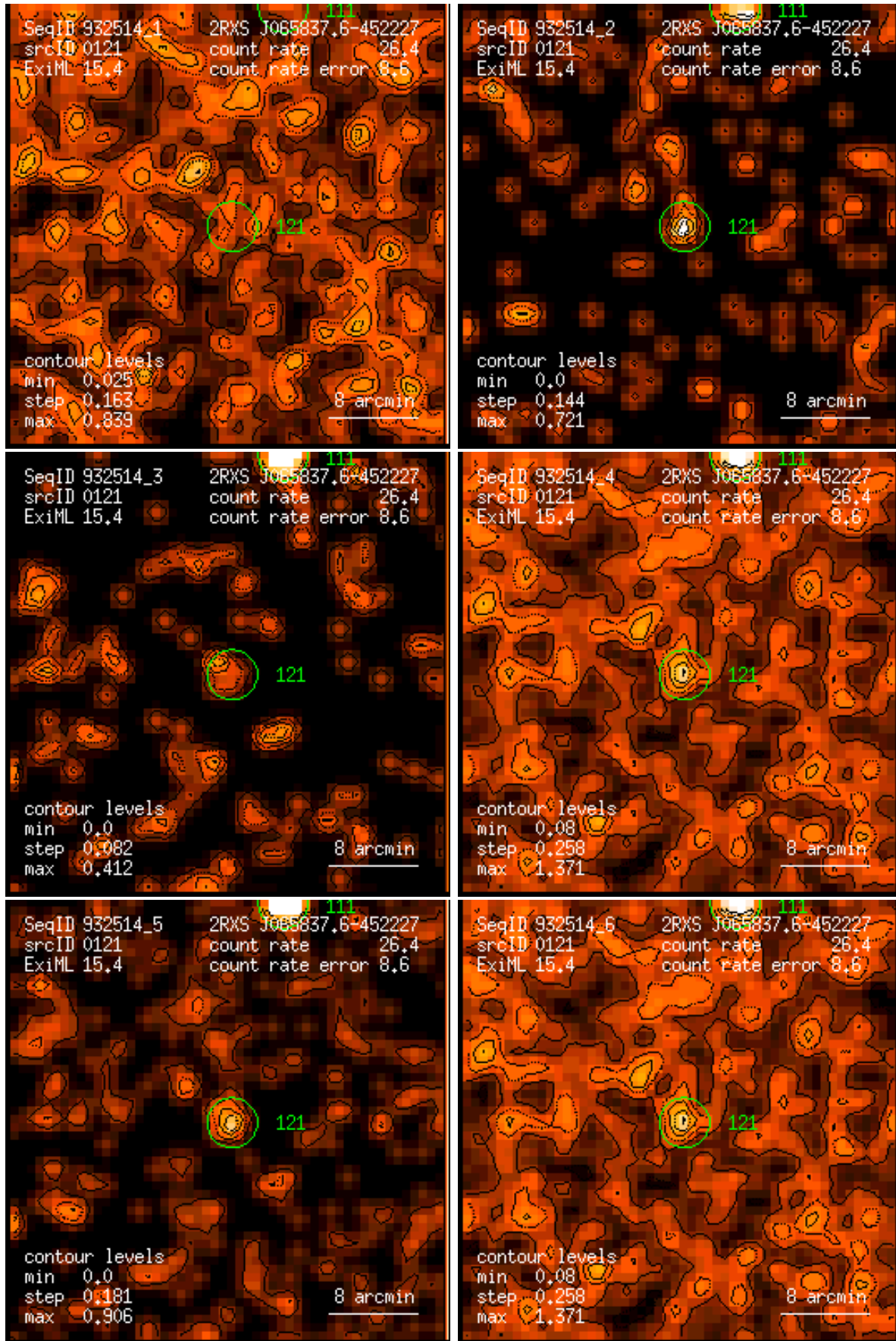
Figure 121: RASS 932514: detection 0121: band rate images, Gaussian filter: (1) PSPC channels 11 – 41, (2) 52 – 90, (3) 91 – 201, (4) 11 – 235, (5) 52 – 201, (6) 11 – 201. Broad band rates in counts/ks. Band rate contour levels in counts/ks/arcmin 2 .
