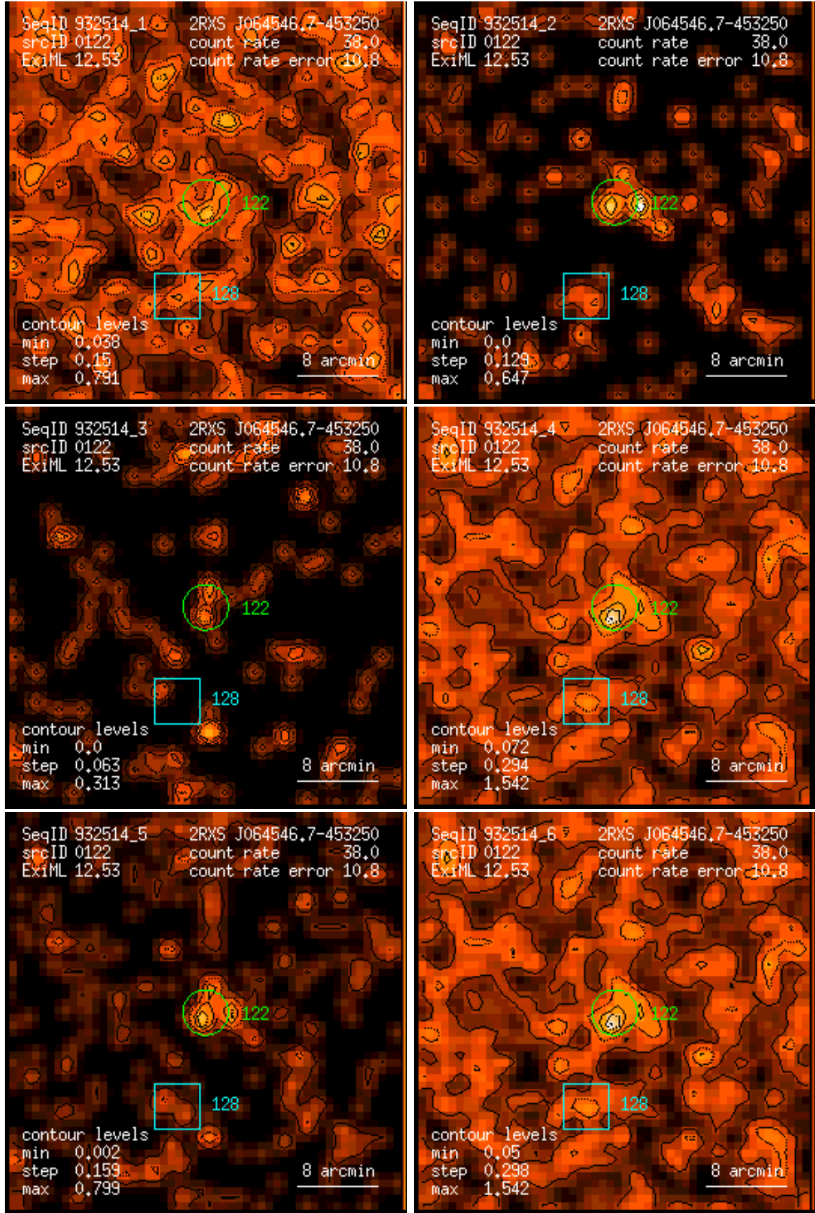
Figure 122: RASS 932514: detection 0122: band rate images, Gaussian filter: (1) PSPC channels 11 – 41, (2) 52 – 90, (3) 91 – 201, (4) 11 – 235, (5) 52 – 201, (6) 11 – 201. Broad band rates in counts/ks. Band rate contour levels in counts/ks/arcmin 2 .
