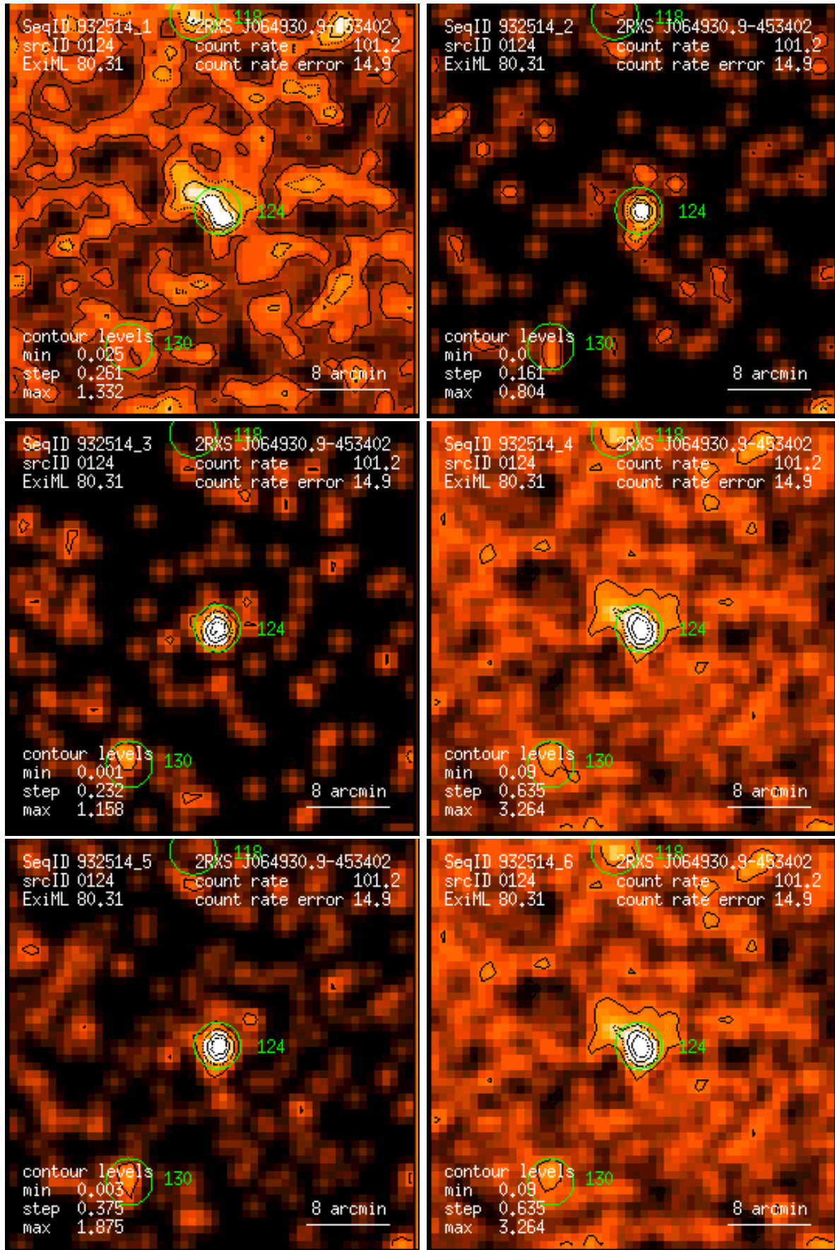
Figure 124: RASS 932514: detection 0124: band rate images, Gaussian filter: (1) PSPC channels 11 – 41, (2) 52 – 90, (3) 91 – 201, (4) 11 – 235, (5) 52 – 201, (6) 11 – 201. Broad band rates in counts/ks. Band rate contour levels in counts/ks/arcmin 2 .
