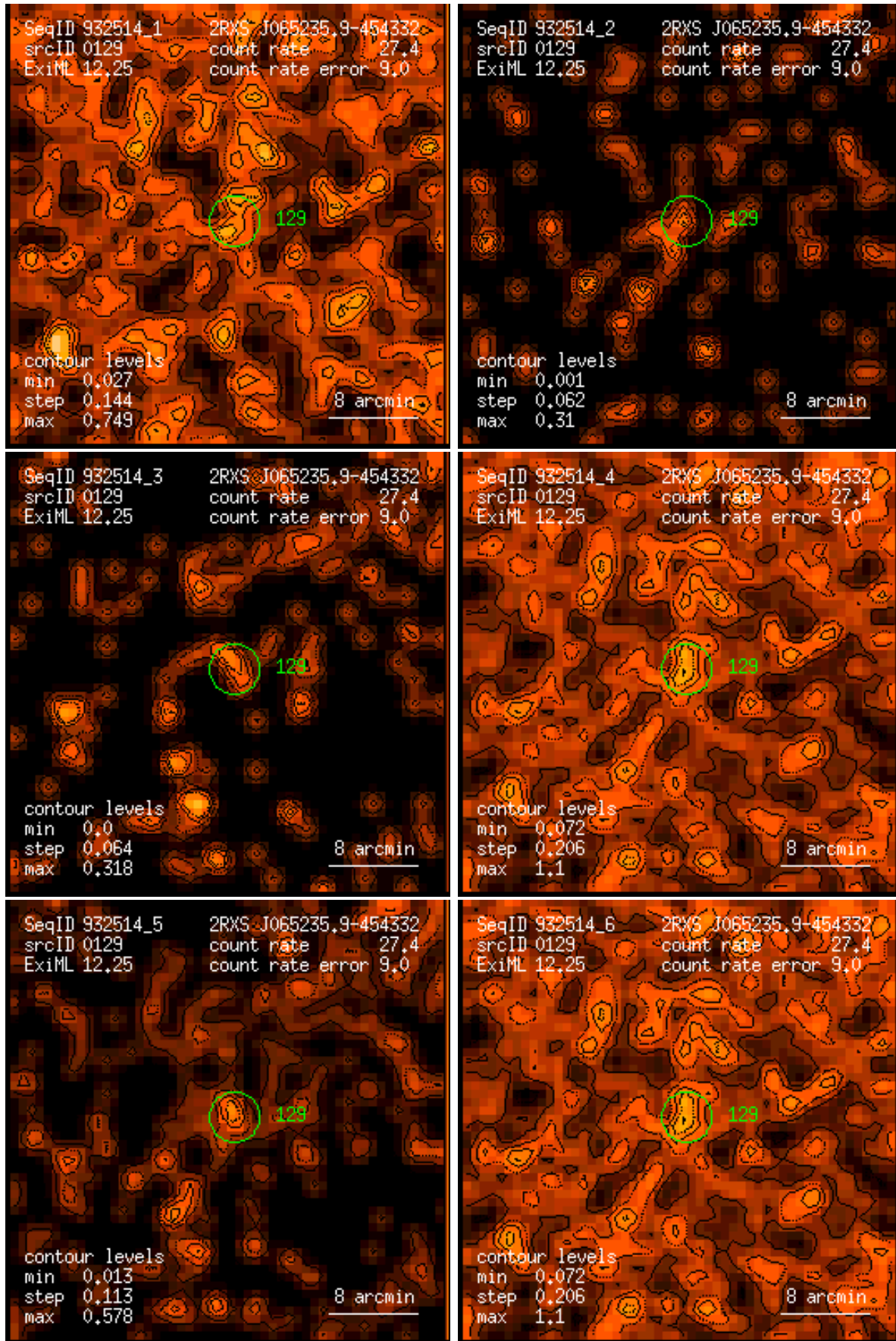
Figure 129: RASS 932514: detection 0129: band rate images, Gaussian filter: (1) PSPC channels 11 – 41, (2) 52 – 90, (3) 91 – 201, (4) 11 – 235, (5) 52 – 201, (6) 11 – 201. Broad band rates in counts/ks. Band rate contour levels in counts/ks/arcmin 2 .
