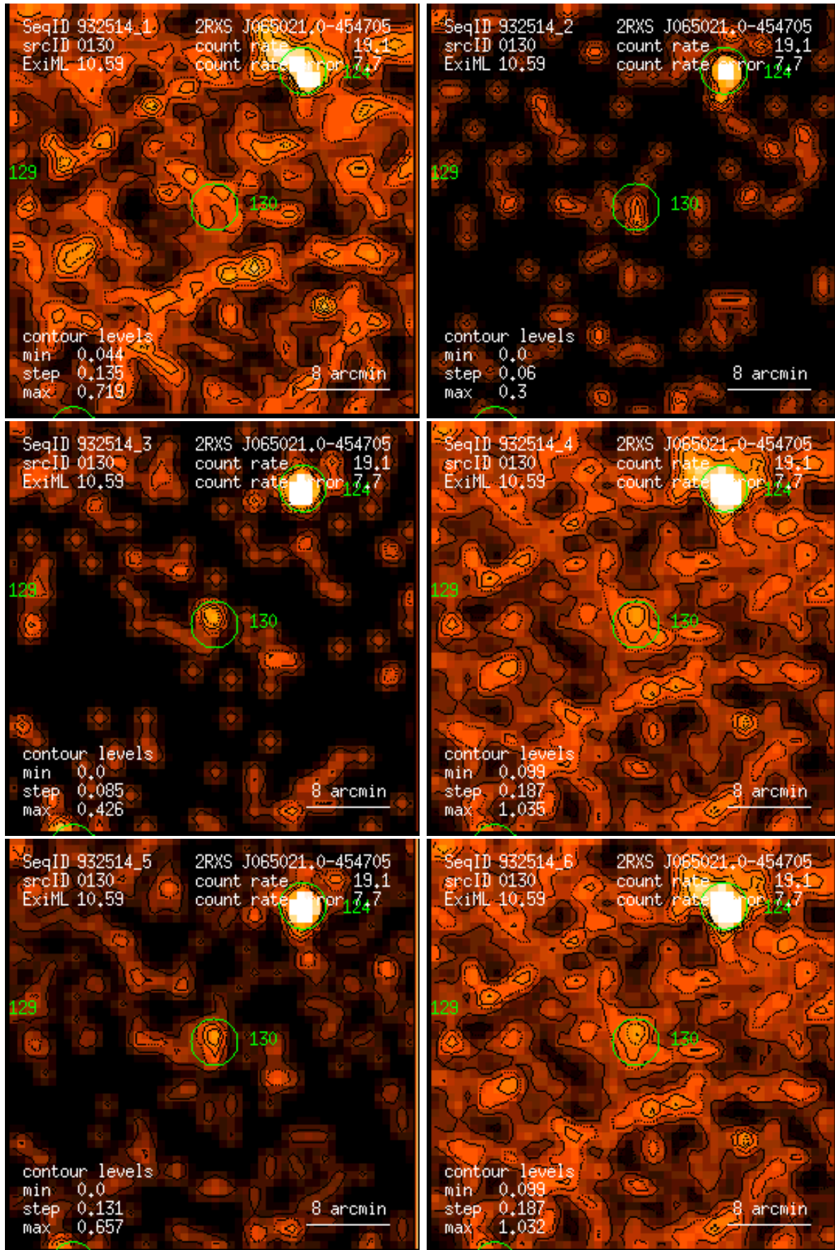
Figure 130: RASS 932514: detection 0130: band rate images, Gaussian filter: (1) PSPC channels 11 – 41, (2) 52 – 90, (3) 91 – 201, (4) 11 – 235, (5) 52 – 201, (6) 11 – 201. Broad band rates in counts/ks. Band rate contour levels in counts/ks/arcmin 2 .
