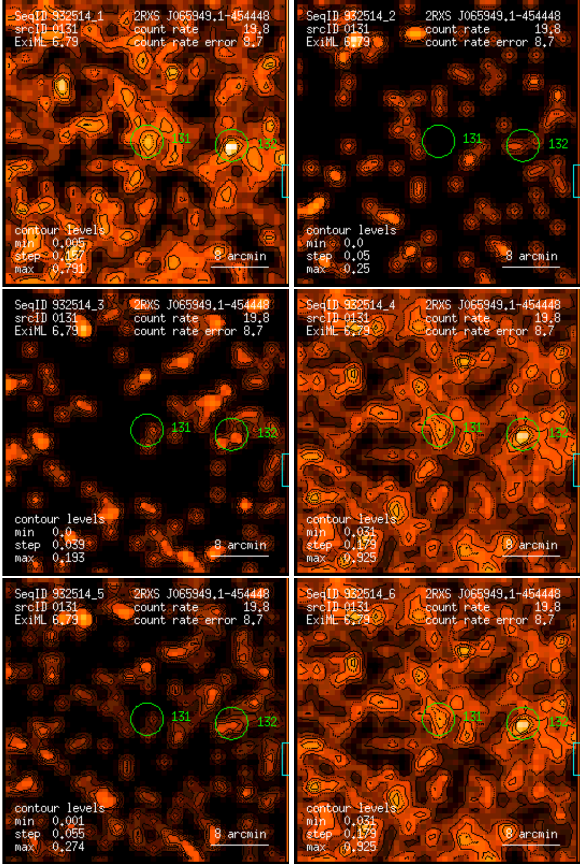
Figure 131: RASS 932514: detection 0131: band rate images, Gaussian filter: (1) PSPC channels 11 – 41, (2) 52 – 90, (3) 91 – 201, (4) 11 – 235, (5) 52 – 201, (6) 11 – 201. Broad band rates in counts/ks. Band rate contour levels in counts/ks/arcmin 2 .
