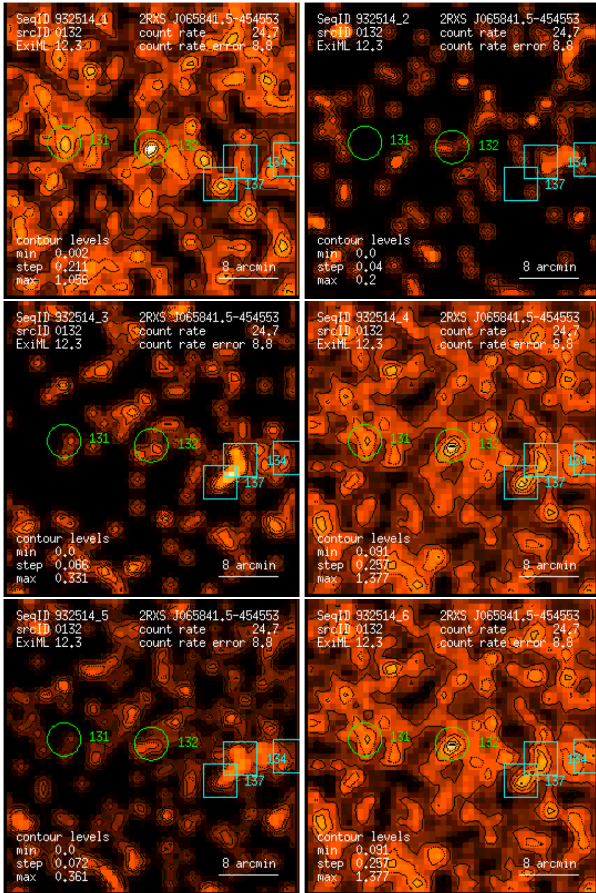
Figure 132: RASS 932514: detection 0132: band rate images, Gaussian filter: (1) PSPC channels 11 – 41, (2) 52 – 90, (3) 91 – 201, (4) 11 – 235, (5) 52 – 201, (6) 11 – 201. Broad band rates in counts/ks. Band rate contour levels in counts/ks/arcmin 2 .
