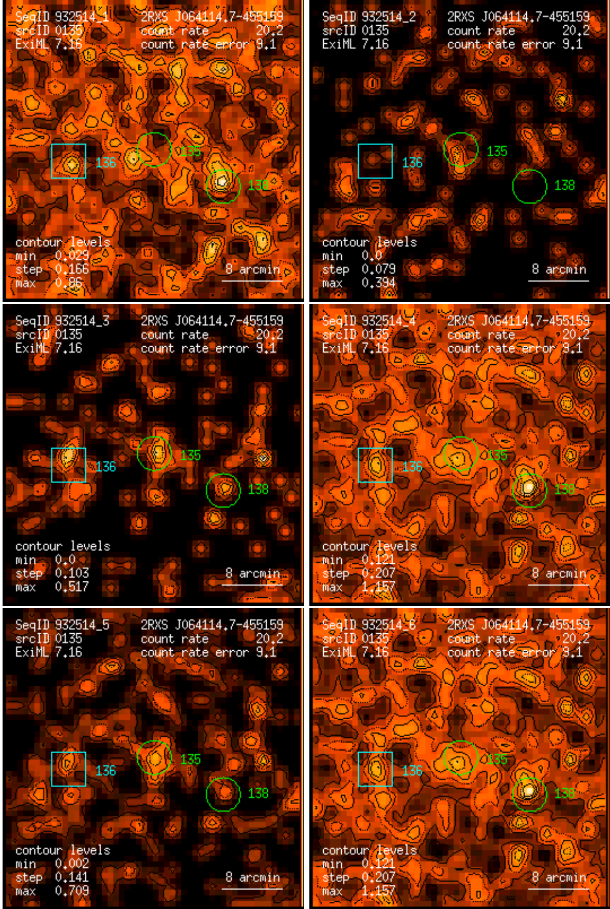
Figure 135: RASS 932514: detection 0135: band rate images, Gaussian filter: (1) PSPC channels 11 – 41, (2) 52 – 90, (3) 91 – 201, (4) 11 – 235, (5) 52 – 201, (6) 11 – 201. Broad band rates in counts/ks. Band rate contour levels in counts/ks/arcmin 2 .
