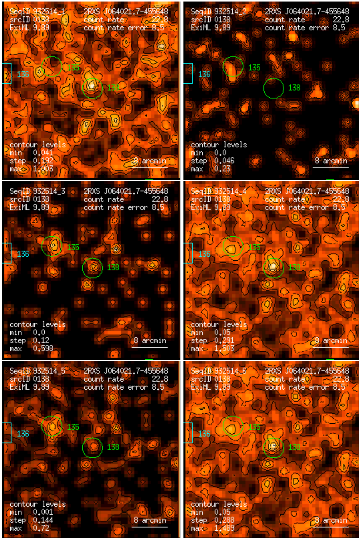
Figure 138: RASS 932514: detection 0138: band rate images, Gaussian filter: (1) PSPC channels 11 – 41, (2) 52 – 90, (3) 91 – 201, (4) 11 – 235, (5) 52 – 201, (6) 11 – 201. Broad band rates in counts/ks. Band rate contour levels in counts/ks/arcmin 2 .
