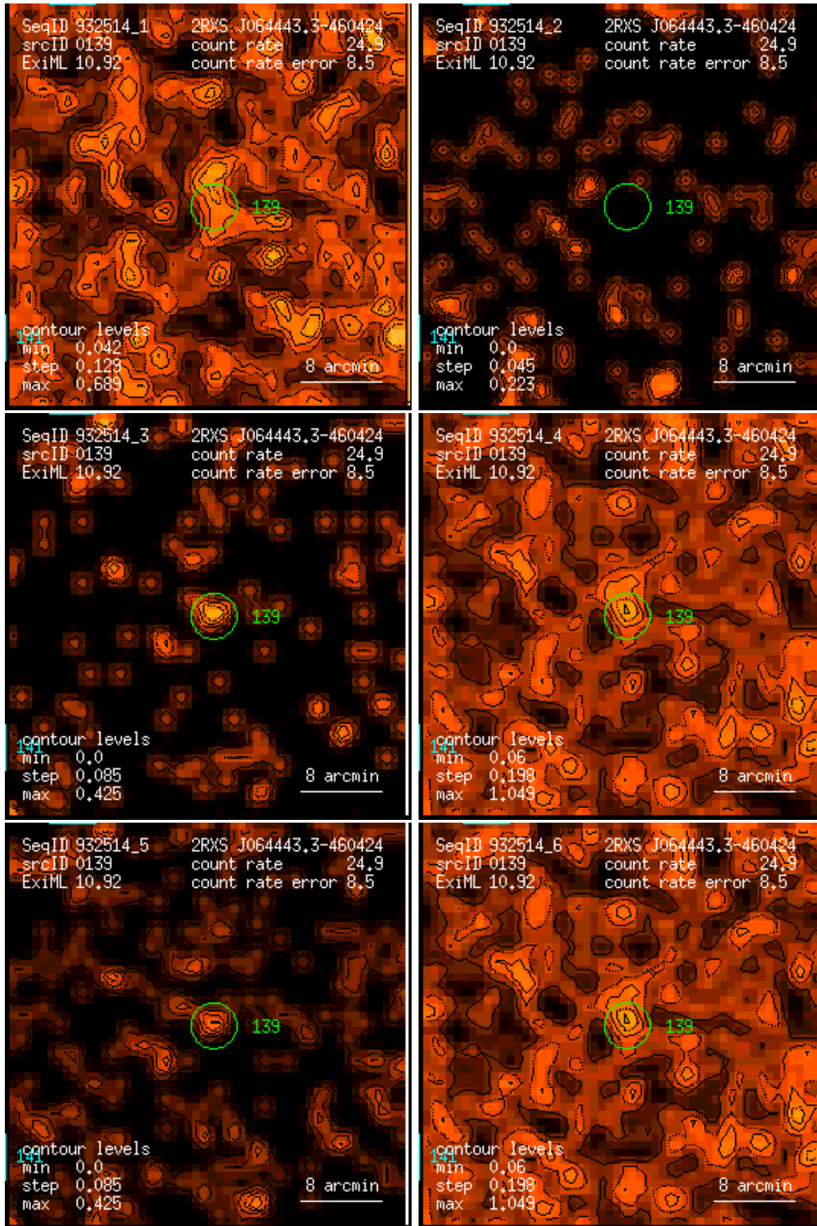
Figure 139: RASS 932514: detection 0139: band rate images, Gaussian filter: (1) PSPC channels 11 – 41, (2) 52 – 90, (3) 91 – 201, (4) 11 – 235, (5) 52 – 201, (6) 11 – 201. Broad band rates in counts/ks. Band rate contour levels in counts/ks/arcmin 2 .
