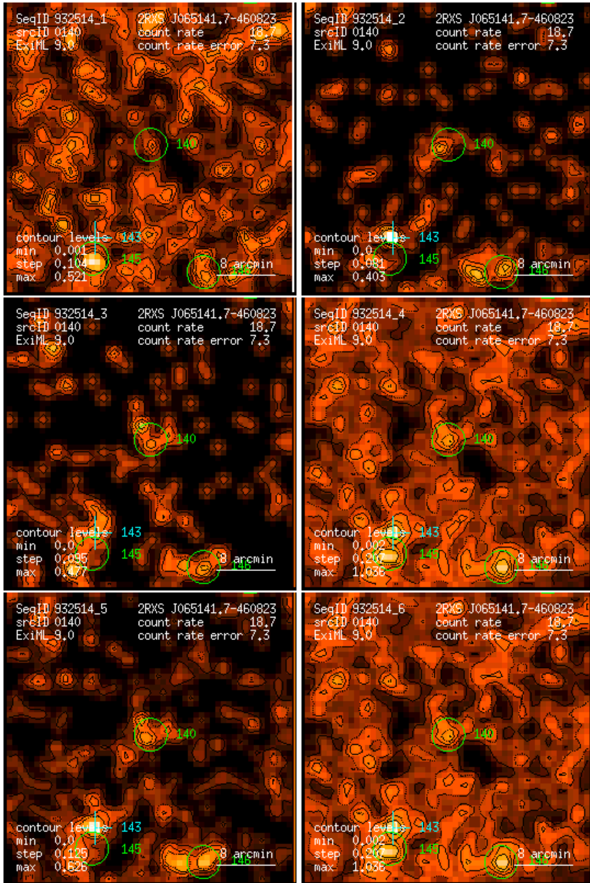
Figure 140: RASS 932514: detection 0140: band rate images, Gaussian filter: (1) PSPC channels 11 – 41, (2) 52 – 90, (3) 91 – 201, (4) 11 – 235, (5) 52 – 201, (6) 11 – 201. Broad band rates in counts/ks. Band rate contour levels in counts/ks/arcmin 2 .
