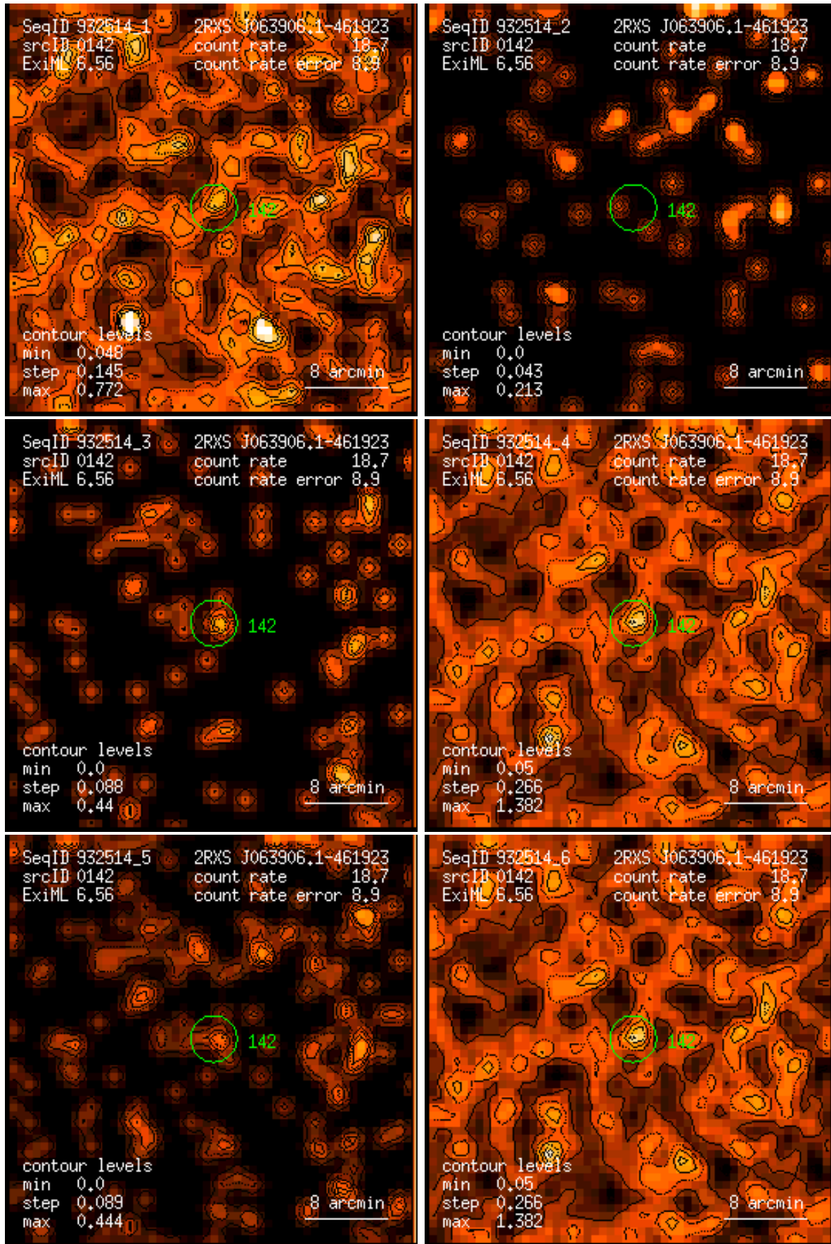
Figure 142: RASS 932514: detection 0142: band rate images, Gaussian filter: (1) PSPC channels 11 – 41, (2) 52 – 90, (3) 91 – 201, (4) 11 – 235, (5) 52 – 201, (6) 11 – 201. Broad band rates in counts/ks. Band rate contour levels in counts/ks/arcmin 2 .
