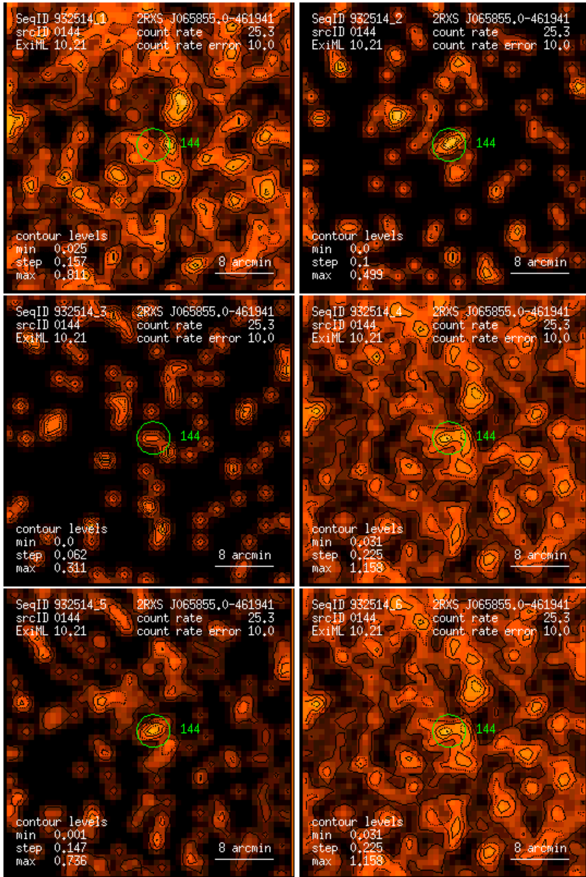
Figure 144: RASS 932514: detection 0144: band rate images, Gaussian filter: (1) PSPC channels 11 – 41, (2) 52 – 90, (3) 91 – 201, (4) 11 – 235, (5) 52 – 201, (6) 11 – 201. Broad band rates in counts/ks. Band rate contour levels in counts/ks/arcmin 2 .
