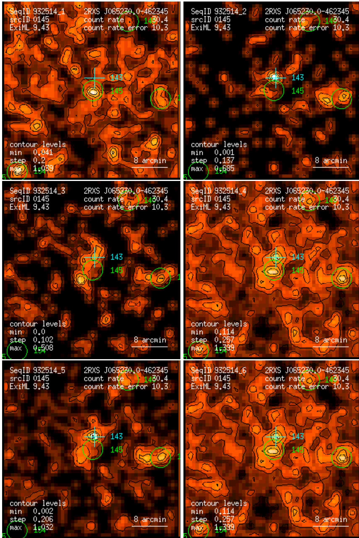
Figure 145: RASS 932514: detection 0145: band rate images, Gaussian filter: (1) PSPC channels 11 – 41, (2) 52 – 90, (3) 91 – 201, (4) 11 – 235, (5) 52 – 201, (6) 11 – 201. Broad band rates in counts/ks. Band rate contour levels in counts/ks/arcmin 2 .
