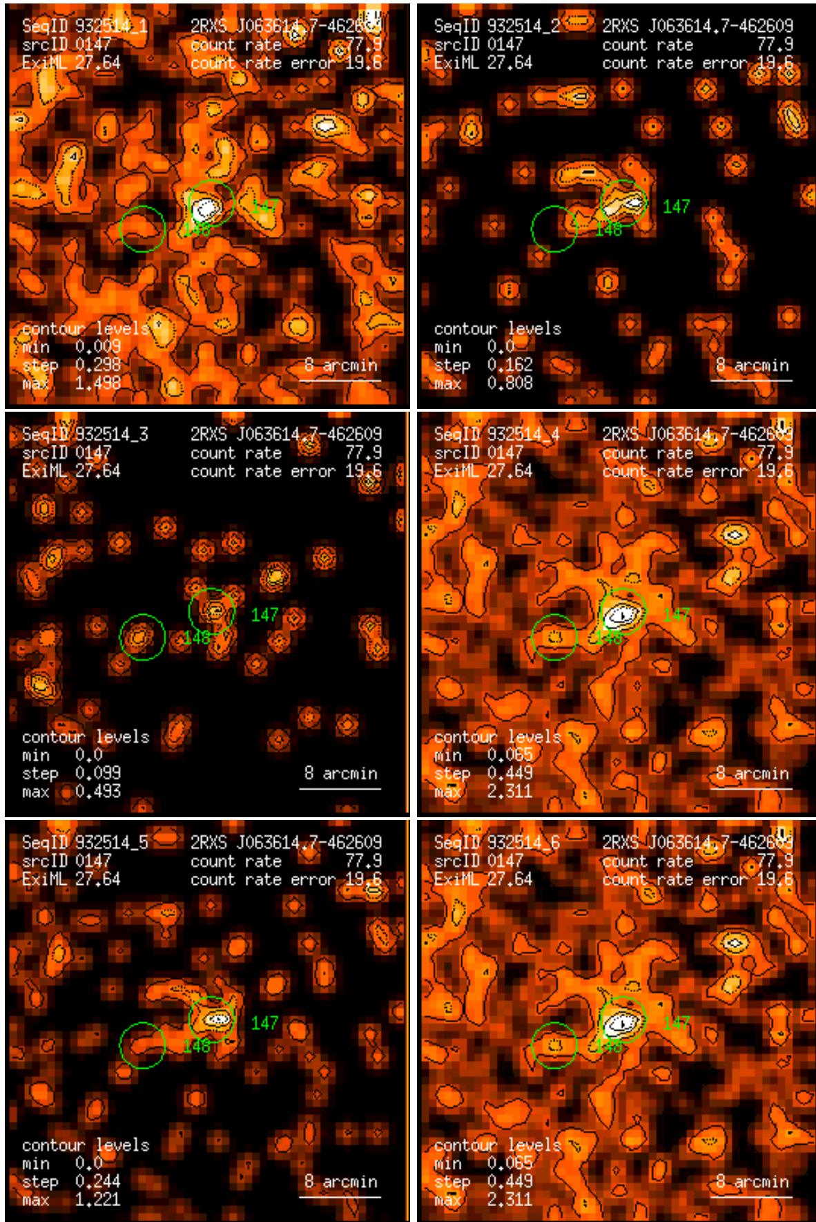
Figure 147: RASS 932514: detection 0147: band rate images, Gaussian filter: (1) PSPC channels 11 – 41, (2) 52 – 90, (3) 91 – 201, (4) 11 – 235, (5) 52 – 201, (6) 11 – 201. Broad band rates in counts/ks. Band rate contour levels in counts/ks/arcmin 2 .
