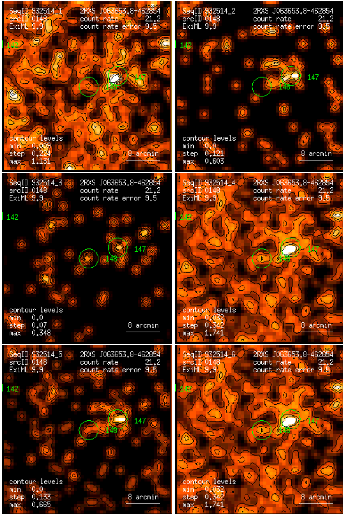
Figure 148: RASS 932514: detection 0148: band rate images, Gaussian filter: (1) PSPC channels 11 – 41, (2) 52 – 90, (3) 91 – 201, (4) 11 – 235, (5) 52 – 201, (6) 11 – 201. Broad band rates in counts/ks. Band rate contour levels in counts/ks/arcmin 2 .
