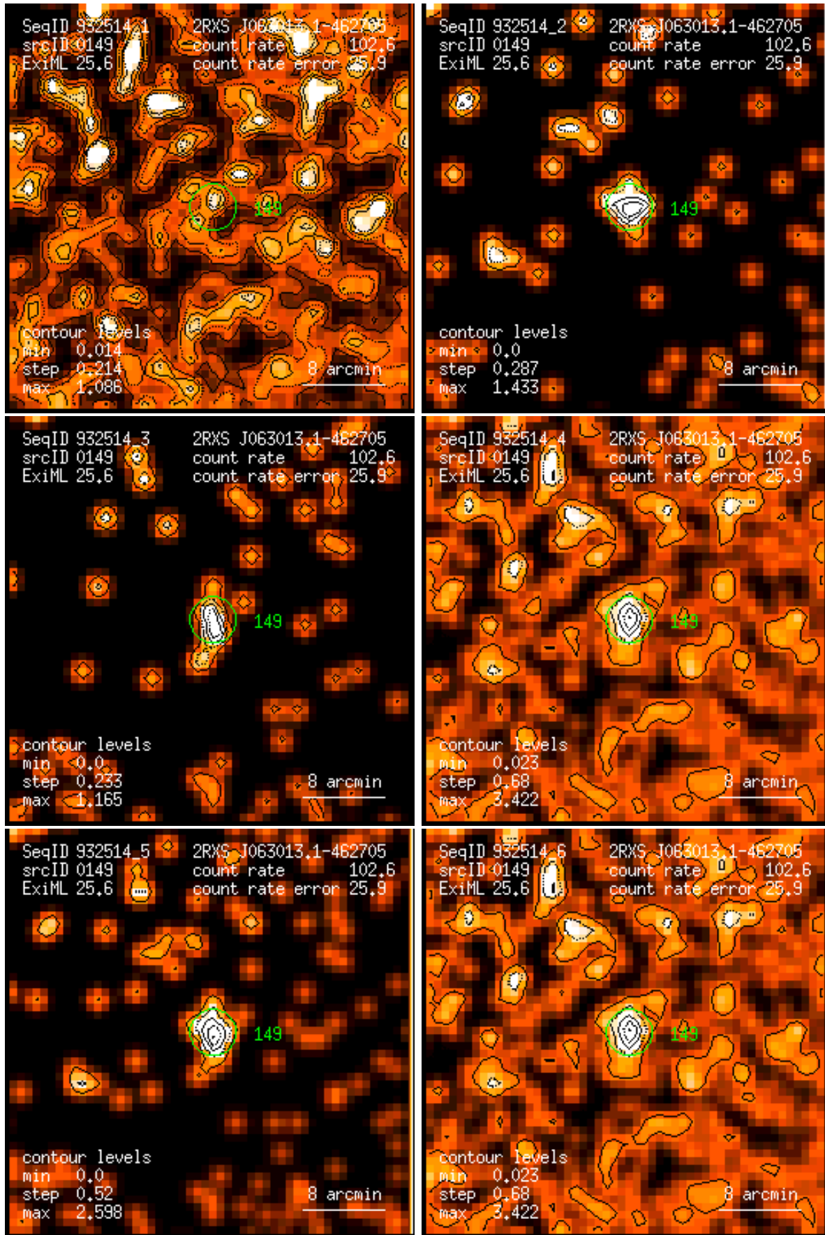
Figure 149: RASS 932514: detection 0149: band rate images, Gaussian filter: (1) PSPC channels 11 – 41, (2) 52 – 90, (3) 91 – 201, (4) 11 – 235, (5) 52 – 201, (6) 11 – 201. Broad band rates in counts/ks. Band rate contour levels in counts/ks/arcmin 2 .
