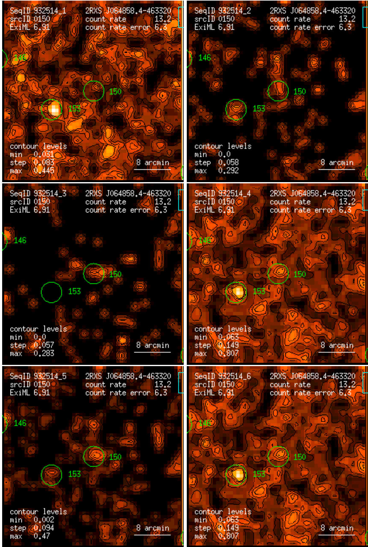
Figure 150: RASS 932514: detection 0150: band rate images, Gaussian filter: (1) PSPC channels 11 – 41, (2) 52 – 90, (3) 91 – 201, (4) 11 – 235, (5) 52 – 201, (6) 11 – 201. Broad band rates in counts/ks. Band rate contour levels in counts/ks/arcmin 2 .
