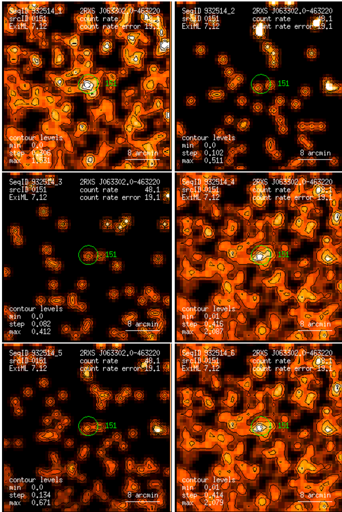
Figure 151: RASS 932514: detection 0151: band rate images, Gaussian filter: (1) PSPC channels 11 – 41, (2) 52 – 90, (3) 91 – 201, (4) 11 – 235, (5) 52 – 201, (6) 11 – 201. Broad band rates in counts/ks. Band rate contour levels in counts/ks/arcmin 2 .
