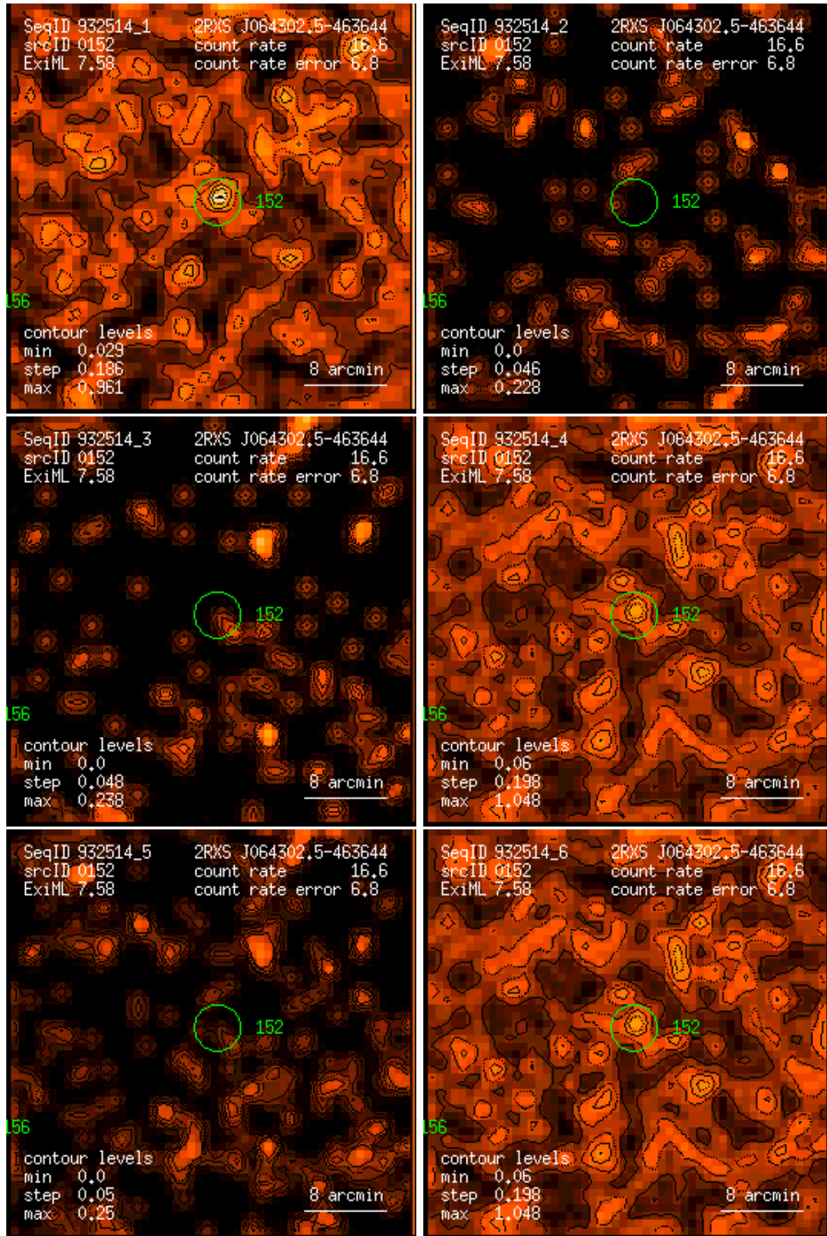
Figure 152: RASS 932514: detection 0152: band rate images, Gaussian filter: (1) PSPC channels 11 – 41, (2) 52 – 90, (3) 91 – 201, (4) 11 – 235, (5) 52 – 201, (6) 11 – 201. Broad band rates in counts/ks. Band rate contour levels in counts/ks/arcmin 2 .
