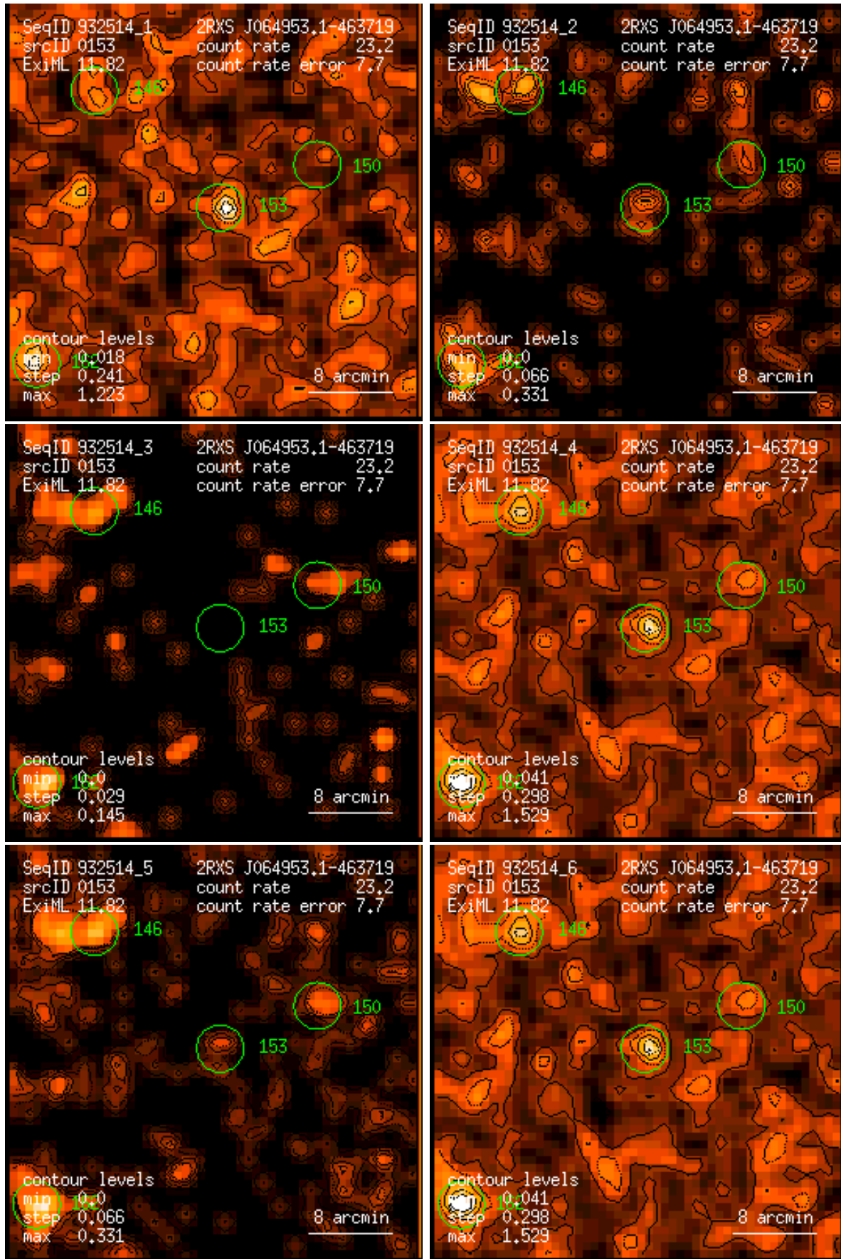
Figure 153: RASS 932514: detection 0153: band rate images, Gaussian filter: (1) PSPC channels 11 – 41, (2) 52 – 90, (3) 91 – 201, (4) 11 – 235, (5) 52 – 201, (6) 11 – 201. Broad band rates in counts/ks. Band rate contour levels in counts/ks/arcmin 2 .
