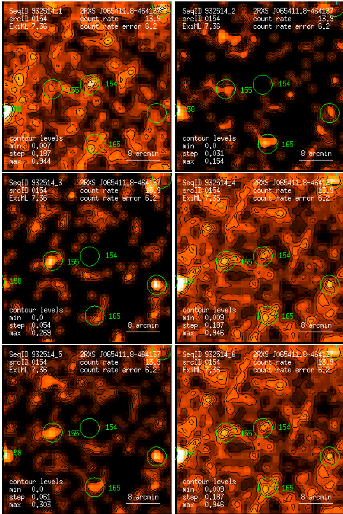
Figure 154: RASS 932514: detection 0154: band rate images, Gaussian filter: (1) PSPC channels 11 – 41, (2) 52 – 90, (3) 91 – 201, (4) 11 – 235, (5) 52 – 201, (6) 11 – 201. Broad band rates in counts/ks. Band rate contour levels in counts/ks/arcmin 2 .
