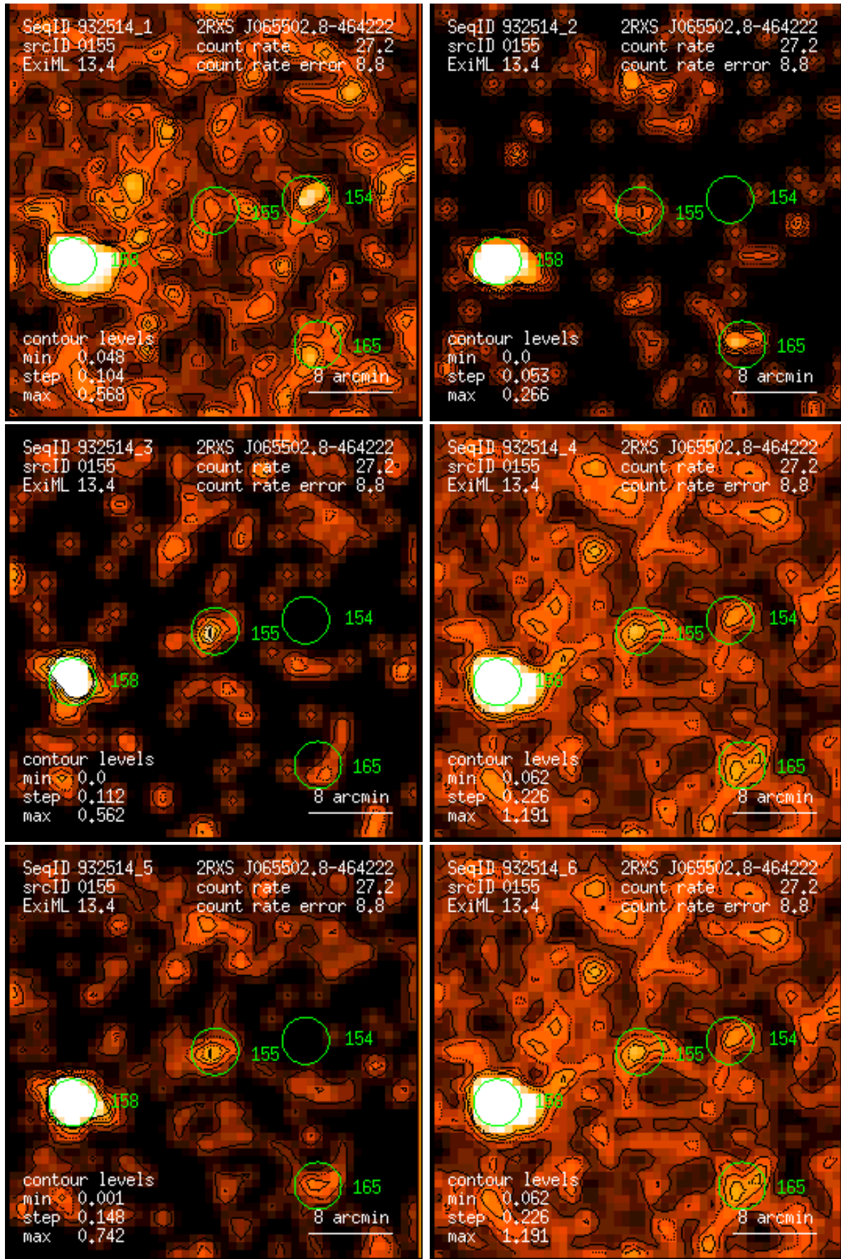
Figure 155: RASS 932514: detection 0155: band rate images, Gaussian filter: (1) PSPC channels 11 – 41, (2) 52 – 90, (3) 91 – 201, (4) 11 – 235, (5) 52 – 201, (6) 11 – 201. Broad band rates in counts/ks. Band rate contour levels in counts/ks/arcmin 2 .
