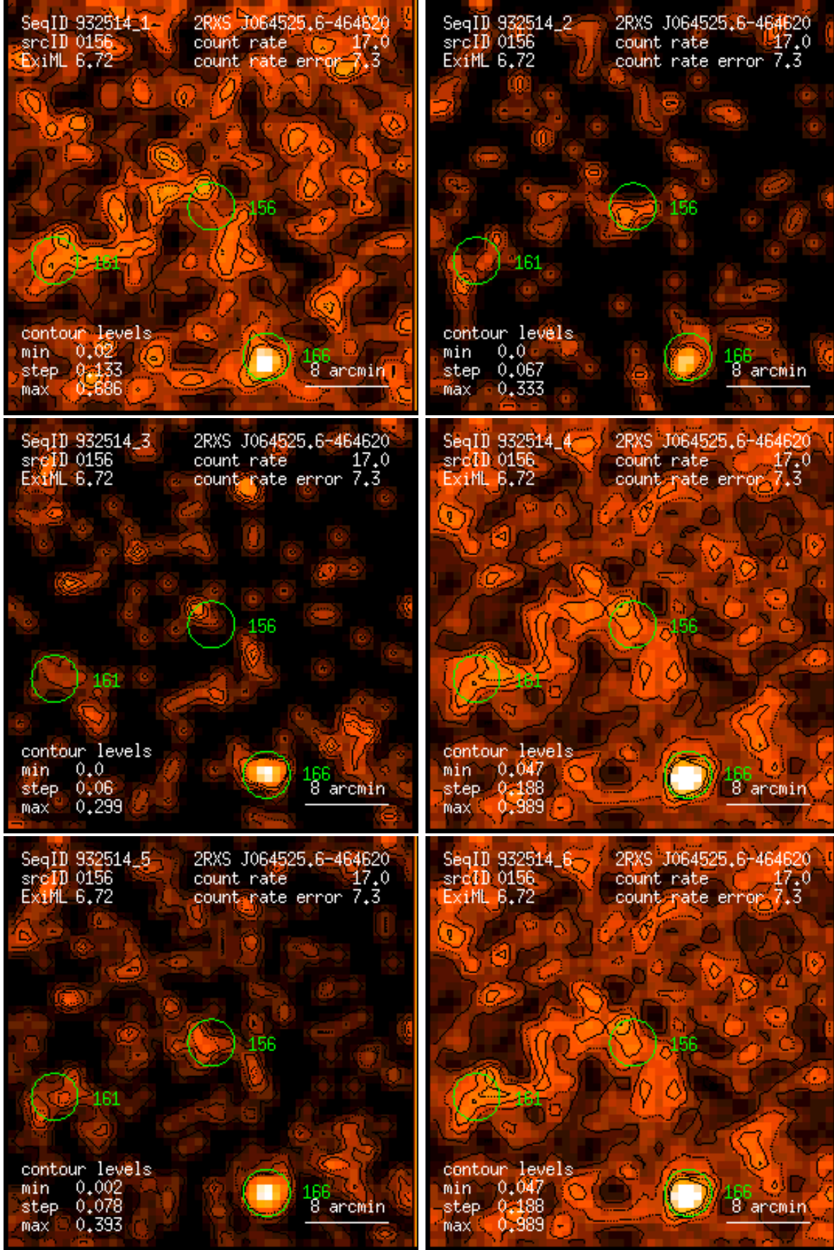
Figure 156: RASS 932514: detection 0156: band rate images, Gaussian filter: (1) PSPC channels 11 – 41, (2) 52 – 90, (3) 91 – 201, (4) 11 – 235, (5) 52 – 201, (6) 11 – 201. Broad band rates in counts/ks. Band rate contour levels in counts/ks/arcmin 2 .
