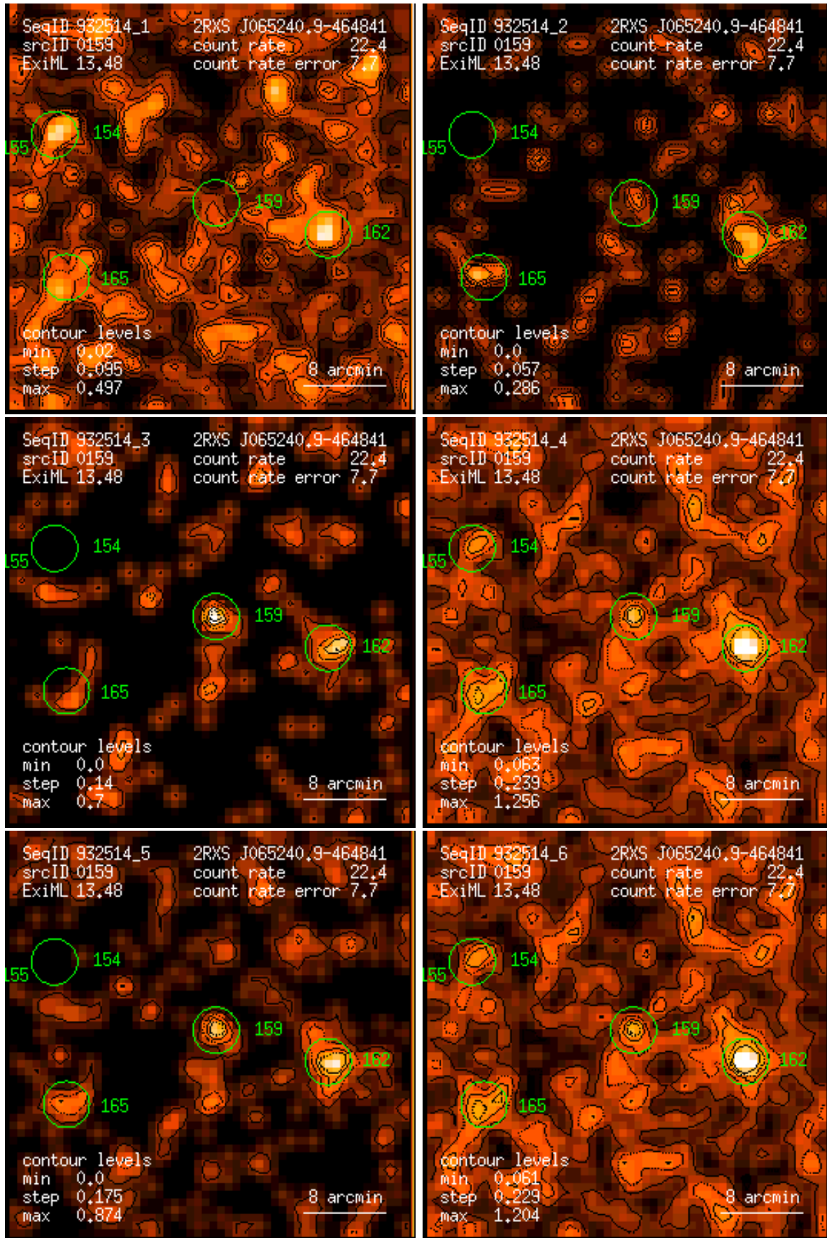
Figure 159: RASS 932514: detection 0159: band rate images, Gaussian filter: (1) PSPC channels 11 – 41, (2) 52 – 90, (3) 91 – 201, (4) 11 – 235, (5) 52 – 201, (6) 11 – 201. Broad band rates in counts/ks. Band rate contour levels in counts/ks/arcmin 2 .
