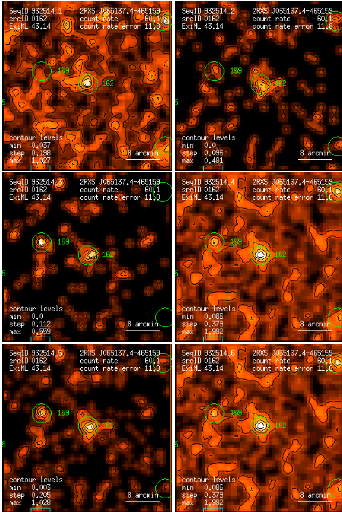
Figure 162: RASS 932514: detection 0162: band rate images, Gaussian filter: (1) PSPC channels 11 – 41, (2) 52 – 90, (3) 91 – 201, (4) 11 – 235, (5) 52 – 201, (6) 11 – 201. Broad band rates in counts/ks. Band rate contour levels in counts/ks/arcmin 2 .
