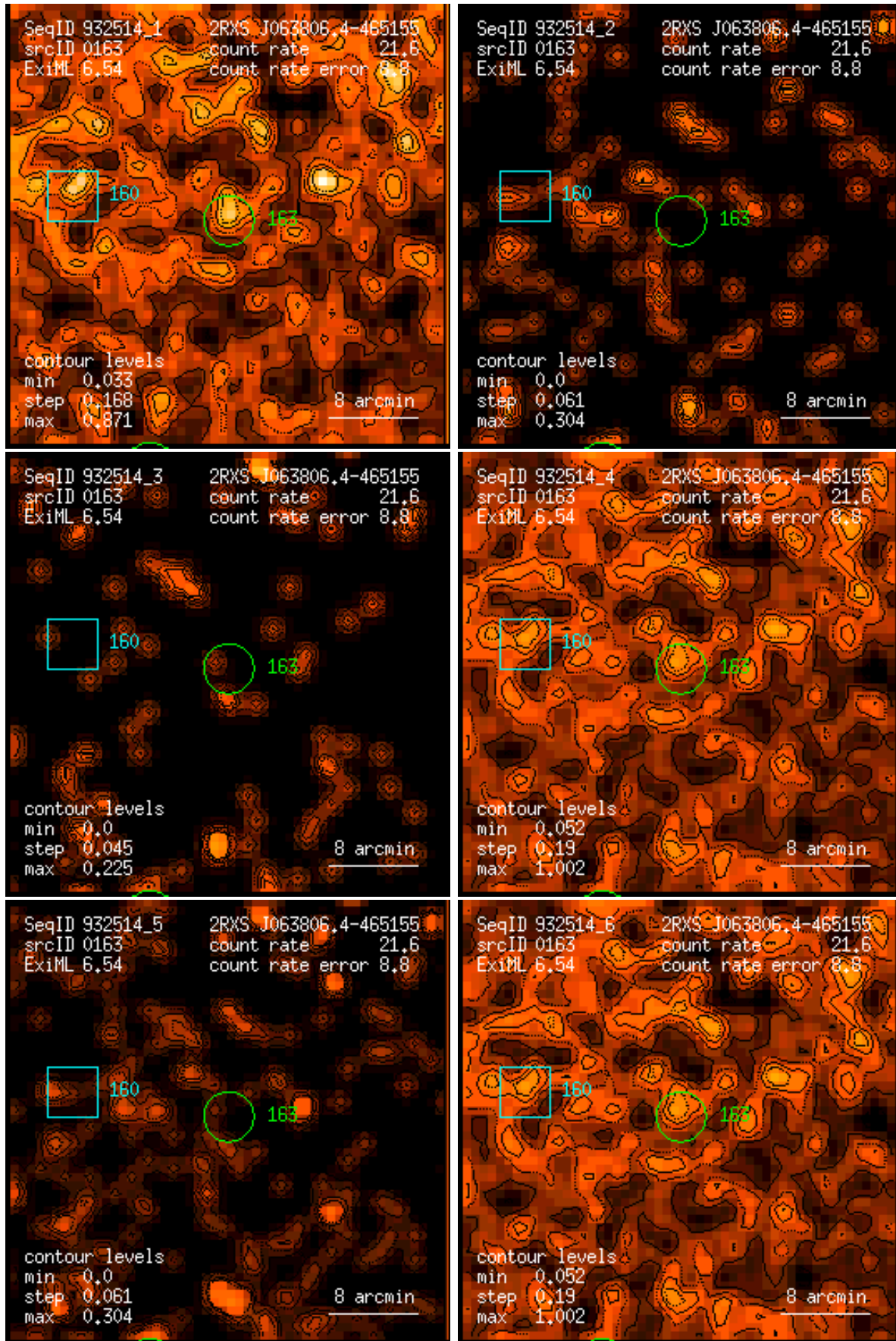
Figure 163: RASS 932514: detection 0163: band rate images, Gaussian filter: (1) PSPC channels 11 – 41, (2) 52 – 90, (3) 91 – 201, (4) 11 – 235, (5) 52 – 201, (6) 11 – 201. Broad band rates in counts/ks. Band rate contour levels in counts/ks/arcmin 2 .
