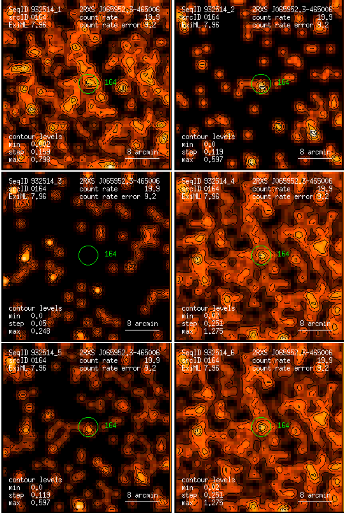
Figure 164: RASS 932514: detection 0164: band rate images, Gaussian filter: (1) PSPC channels 11 – 41, (2) 52 – 90, (3) 91 – 201, (4) 11 – 235, (5) 52 – 201, (6) 11 – 201. Broad band rates in counts/ks. Band rate contour levels in counts/ks/arcmin 2 .
