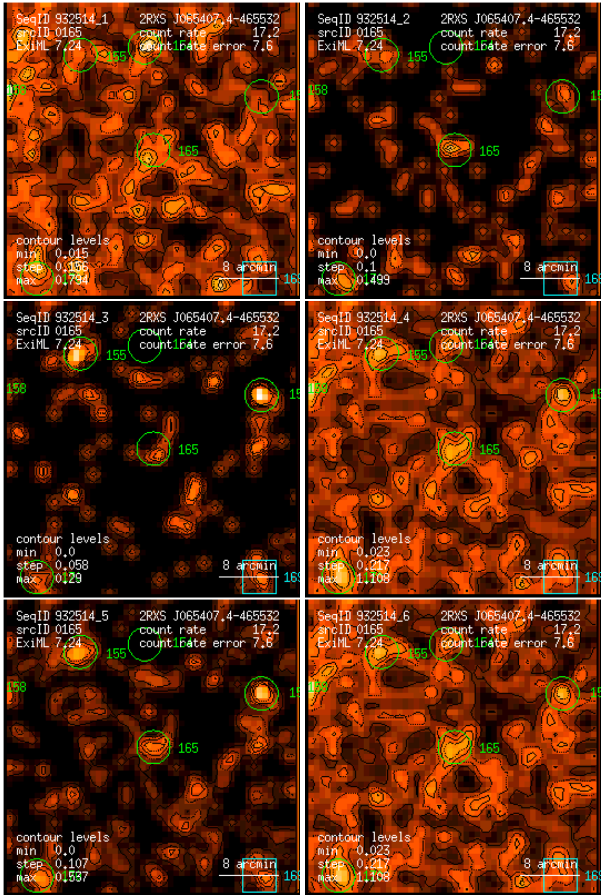
Figure 165: RASS 932514: detection 0165: band rate images, Gaussian filter: (1) PSPC channels 11 – 41, (2) 52 – 90, (3) 91 – 201, (4) 11 – 235, (5) 52 – 201, (6) 11 – 201. Broad band rates in counts/ks. Band rate contour levels in counts/ks/arcmin 2 .
