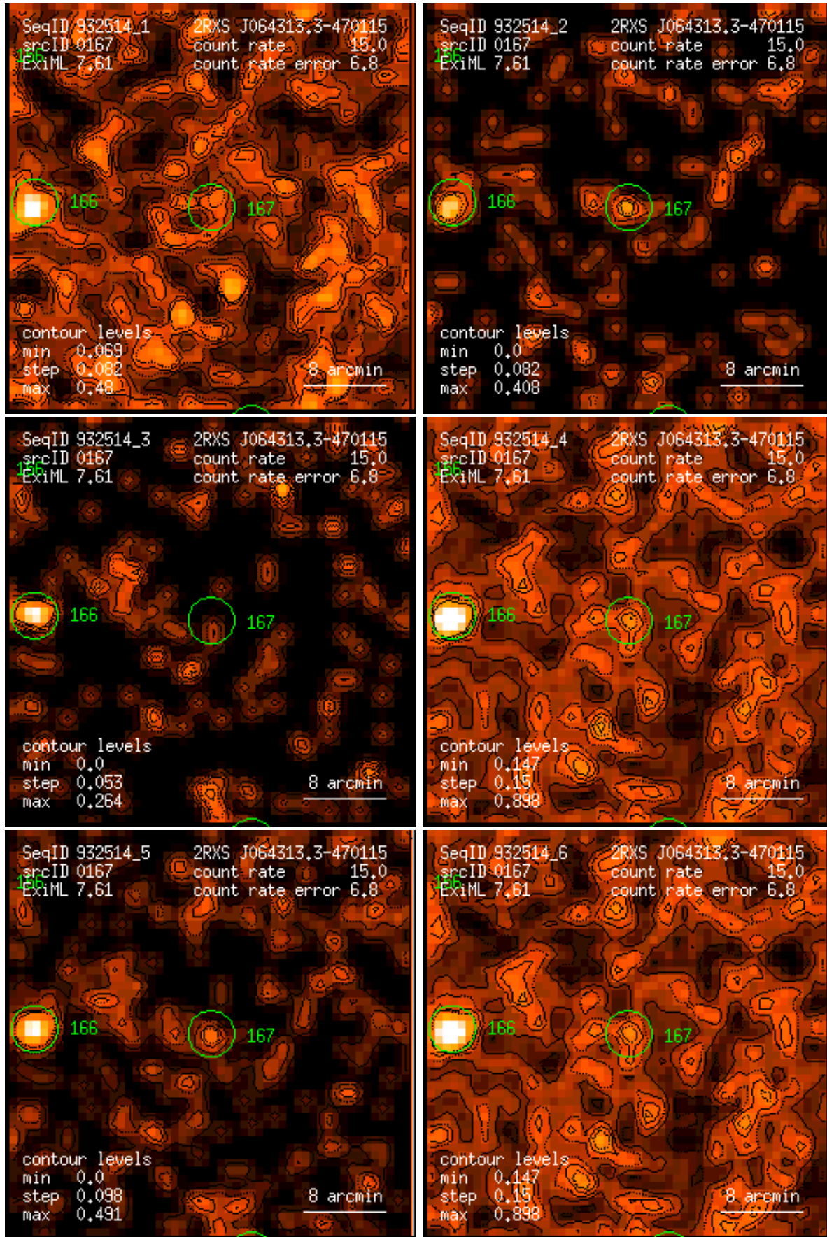
Figure 167: RASS 932514: detection 0167: band rate images, Gaussian filter: (1) PSPC channels 11 – 41, (2) 52 – 90, (3) 91 – 201, (4) 11 – 235, (5) 52 – 201, (6) 11 – 201. Broad band rates in counts/ks. Band rate contour levels in counts/ks/arcmin 2 .
