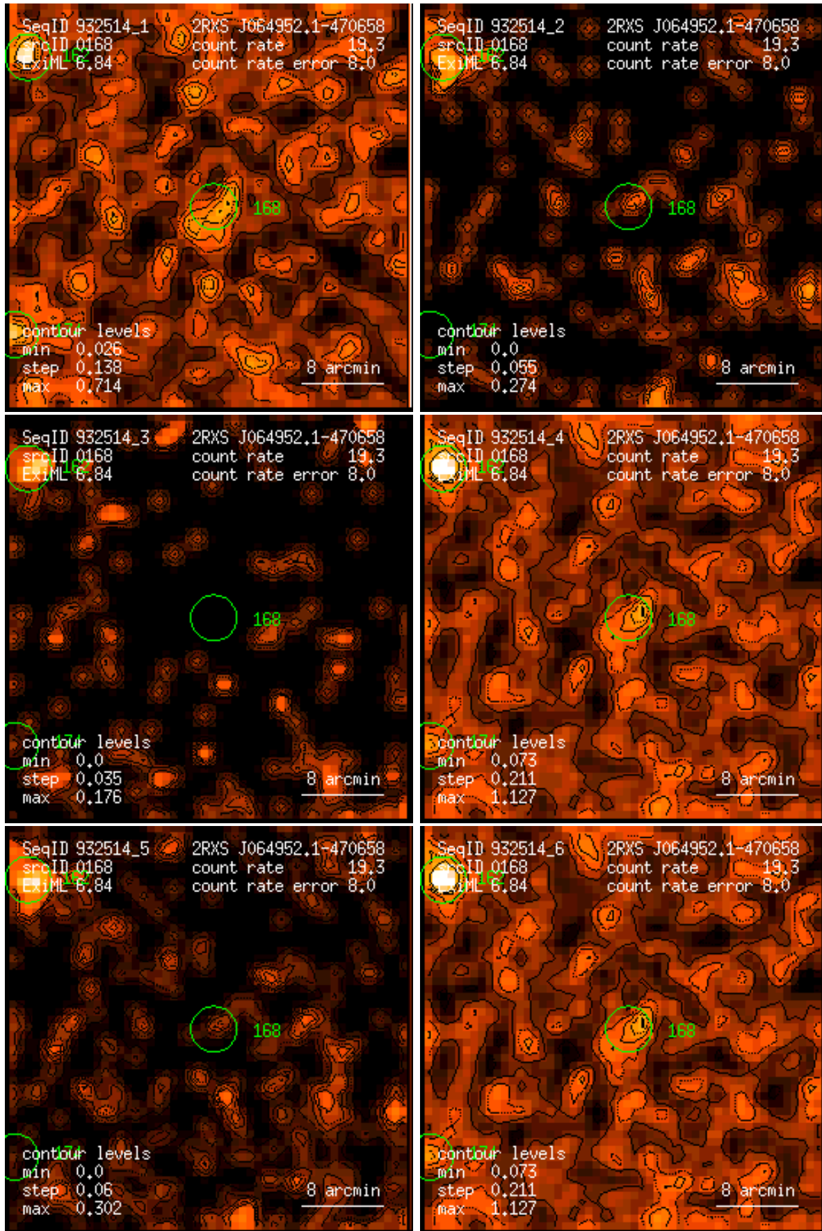
Figure 168: RASS 932514: detection 0168: band rate images, Gaussian filter: (1) PSPC channels 11 – 41, (2) 52 – 90, (3) 91 – 201, (4) 11 – 235, (5) 52 – 201, (6) 11 – 201. Broad band rates in counts/ks. Band rate contour levels in counts/ks/arcmin 2 .
